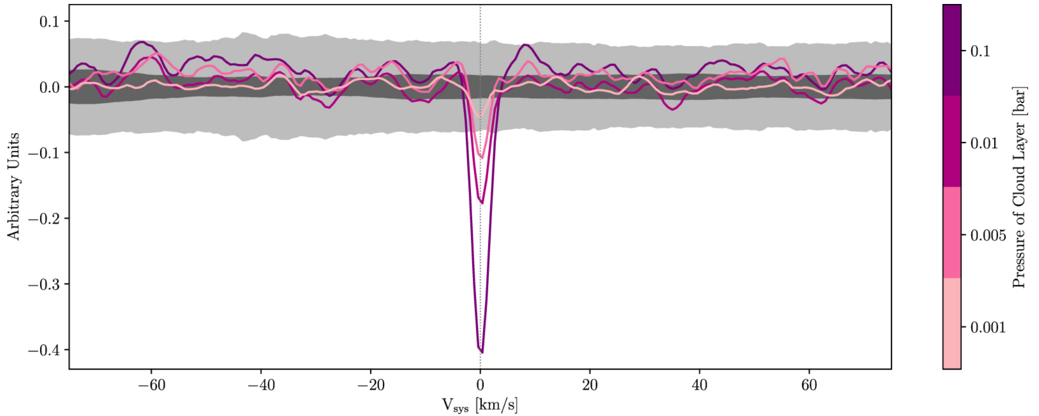
Figure 7. from High-resolution Transit Spectroscopy of Warm Saturns null 2019 AJ 157 58 doi:10.3847/1538-3881/aaf56b https://dx.doi.org/10.3847/1538-3881/aaf56b © 2019. The American Astronomical Society. All rights reserved.
