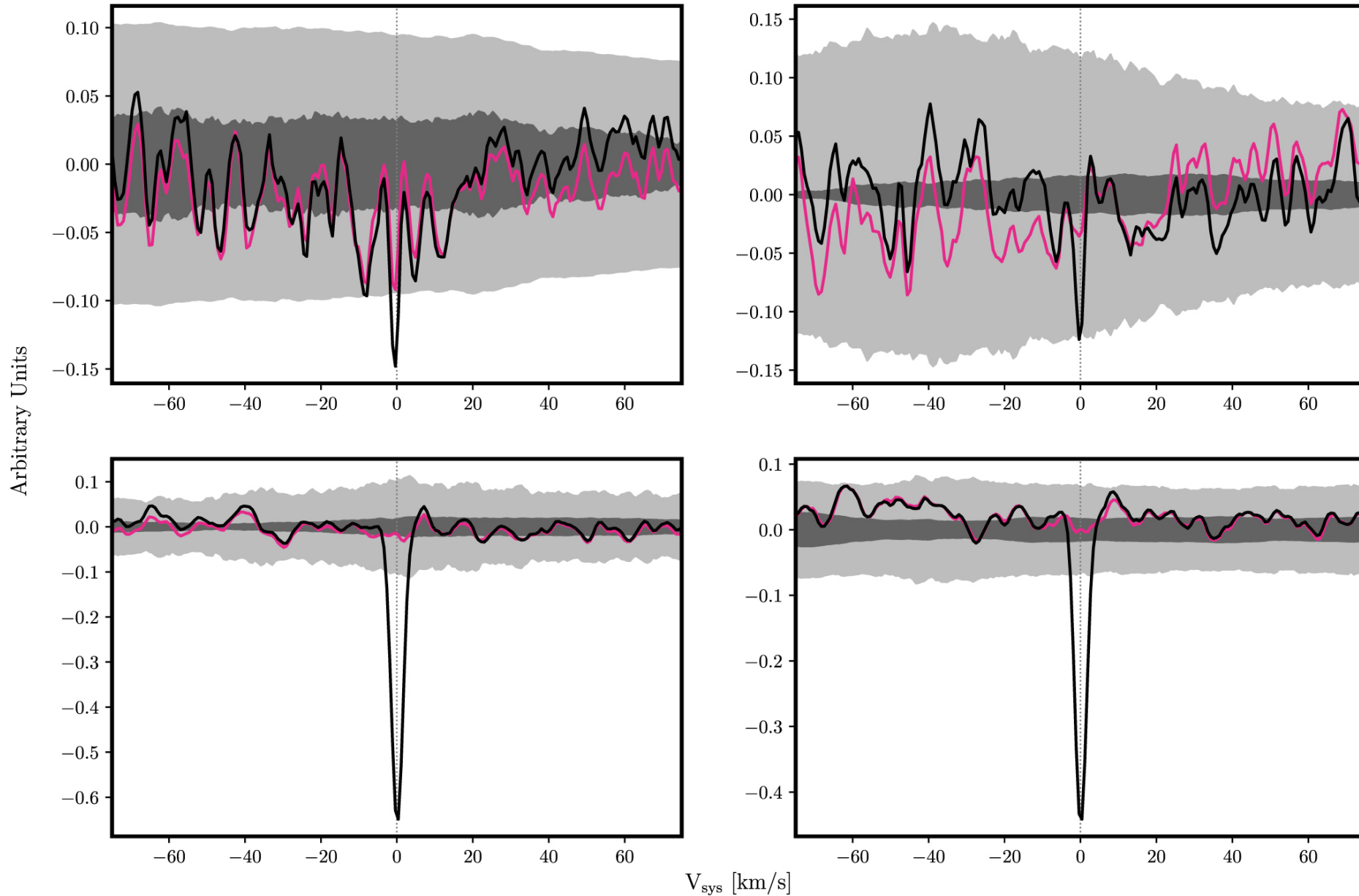
Figure 6. from High-resolution Transit Spectroscopy of Warm Saturns null 2019 AJ 157 58 doi:10.3847/1538-3881/aaf56b https://dx.doi.org/10.3847/1538-3881/aaf56b © 2019. The American Astronomical Society. All rights reserved.
