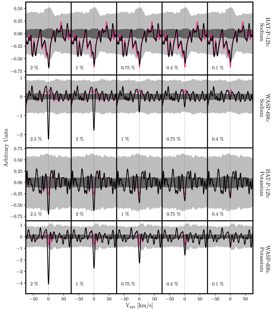
Figure 4. from High-resolution Transit Spectroscopy of Warm Saturns null 2019 AJ 157 58 doi:10.3847/1538-3881/aaf56b https://dx.doi.org/10.3847/1538-3881/aaf56b © 2019. The American Astronomical Society. All rights reserved.
