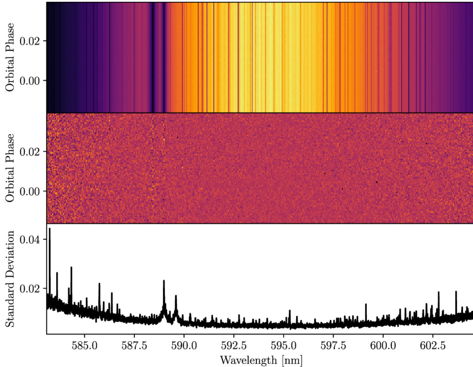
Figure 2. from High-resolution Transit Spectroscopy of Warm Saturns null 2019 AJ 157 58 doi:10.3847/1538-3881/aaf56b https://dx.doi.org/10.3847/1538-3881/aaf56b © 2019. The American Astronomical Society. All rights reserved.
