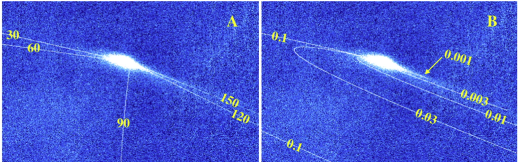
Figure 4. from Active Asteroid P/2017 S5 (ATLAS) null 2019 AJ 157 54 doi:10.3847/1538-3881/aaf563 https://dx.doi.org/10.3847/1538-3881/aaf563 © 2019. The American Astronomical Society. All rights reserved.
