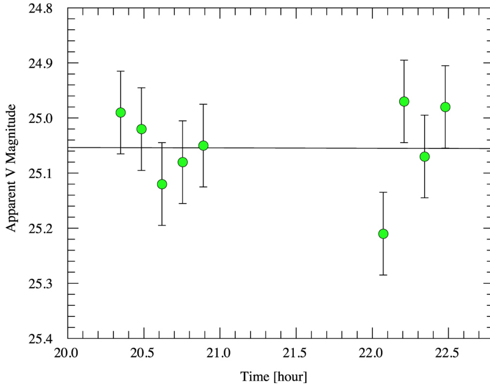
Figure 3. from Active Asteroid P/2017 S5 (ATLAS) null 2019 AJ 157 54 doi:10.3847/1538-3881/aaf563 https://dx.doi.org/10.3847/1538-3881/aaf563
