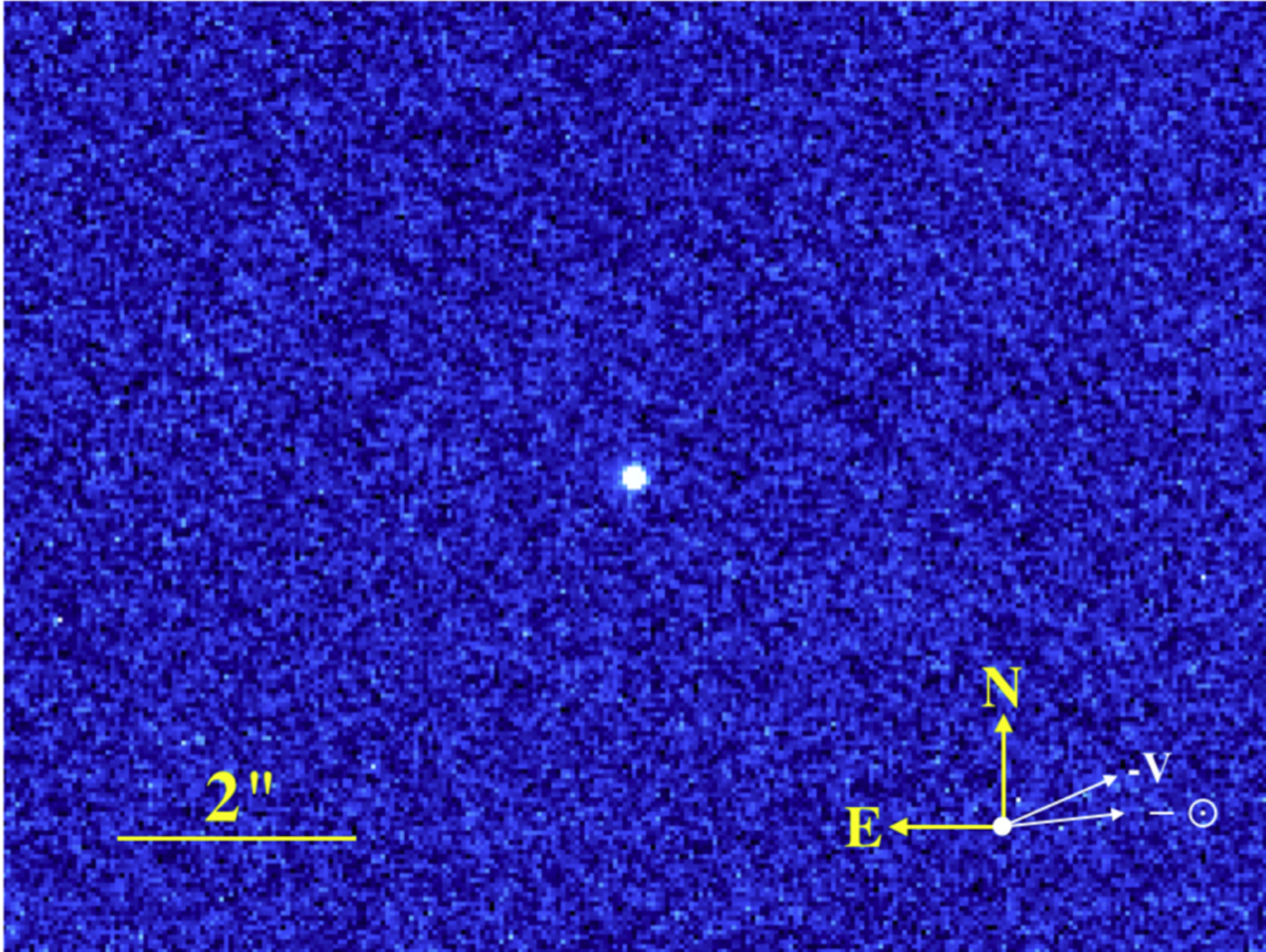
Figure 2. from Active Asteroid P/2017 S5 (ATLAS) null 2019 AJ 157 54 doi:10.3847/1538-3881/aaf563 https://dx.doi.org/10.3847/1538-3881/aaf563 © 2019. The American Astronomical Society. All rights reserved.
