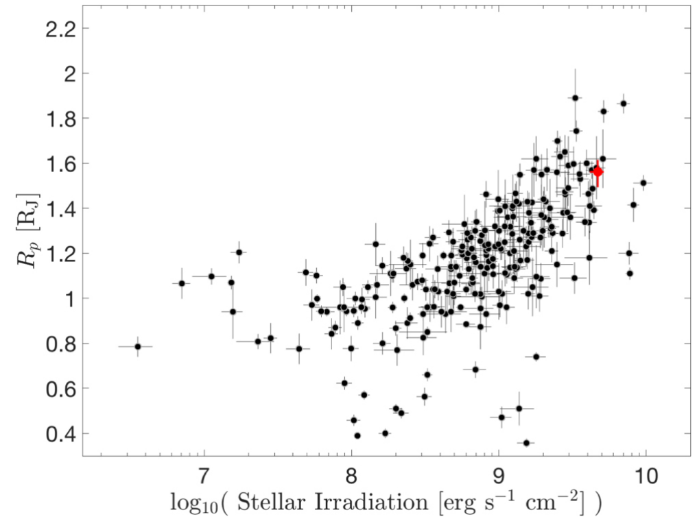
Figure 7. from HD 202772A b: A Transiting Hot Jupiter around a Bright, Mildly Evolved Star in a Visual Binary Discovered by TESS null 2019 AJ 157 51 doi:10.3847/1538-3881/aaf1b7 https://dx.doi.org/10.3847/1538-3881/aaf1b7 © 2019. The American Astronomical Society. All rights reserved.
