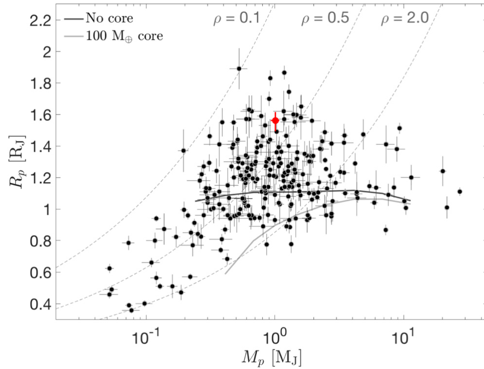
Figure 7. from HD 202772A b: A Transiting Hot Jupiter around a Bright, Mildly Evolved Star in a Visual Binary Discovered by TESS null 2019 AJ 157 51 doi:10.3847/1538-3881/aaf1b7 https://dx.doi.org/10.3847/1538-3881/aaf1b7 © 2019. The American Astronomical Society. All rights reserved.
