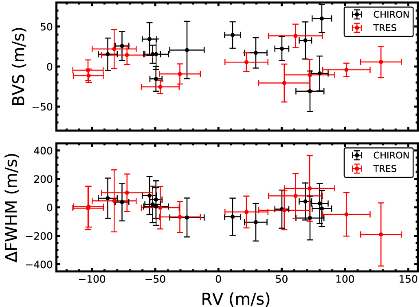
Figure 6. from HD 202772A b: A Transiting Hot Jupiter around a Bright, Mildly Evolved Star in a Visual Binary Discovered by TESS null 2019 AJ 157 51 doi:10.3847/1538-3881/aaf1b7 https://dx.doi.org/10.3847/1538-3881/aaf1b7 © 2019. The American Astronomical Society. All rights reserved.
