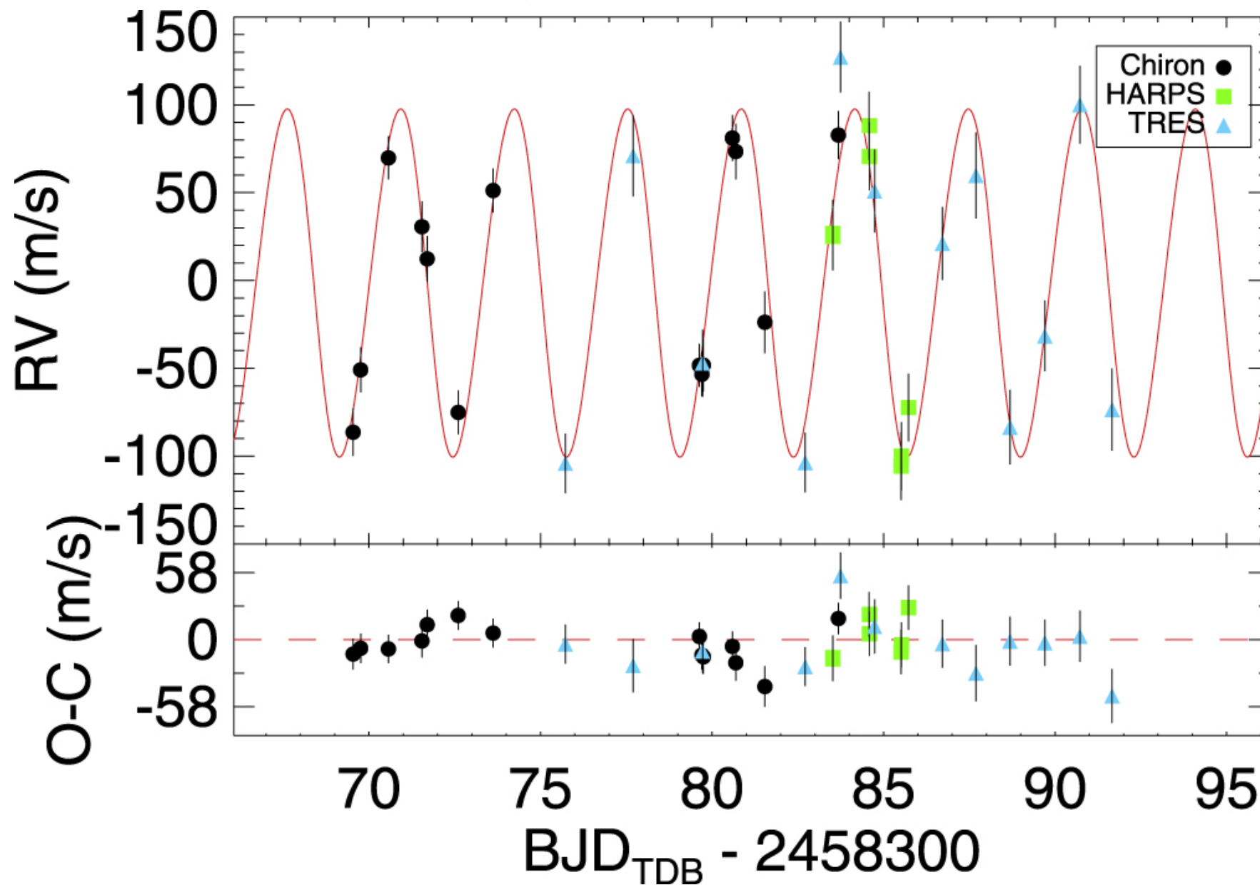
Figure 5. from HD 202772A b: A Transiting Hot Jupiter around a Bright, Mildly Evolved Star in a Visual Binary Discovered by TESS null 2019 AJ 157 51 doi:10.3847/1538-3881/aaf1b7 https://dx.doi.org/10.3847/1538-3881/aaf1b7 © 2019. The American Astronomical Society. All rights reserved.
