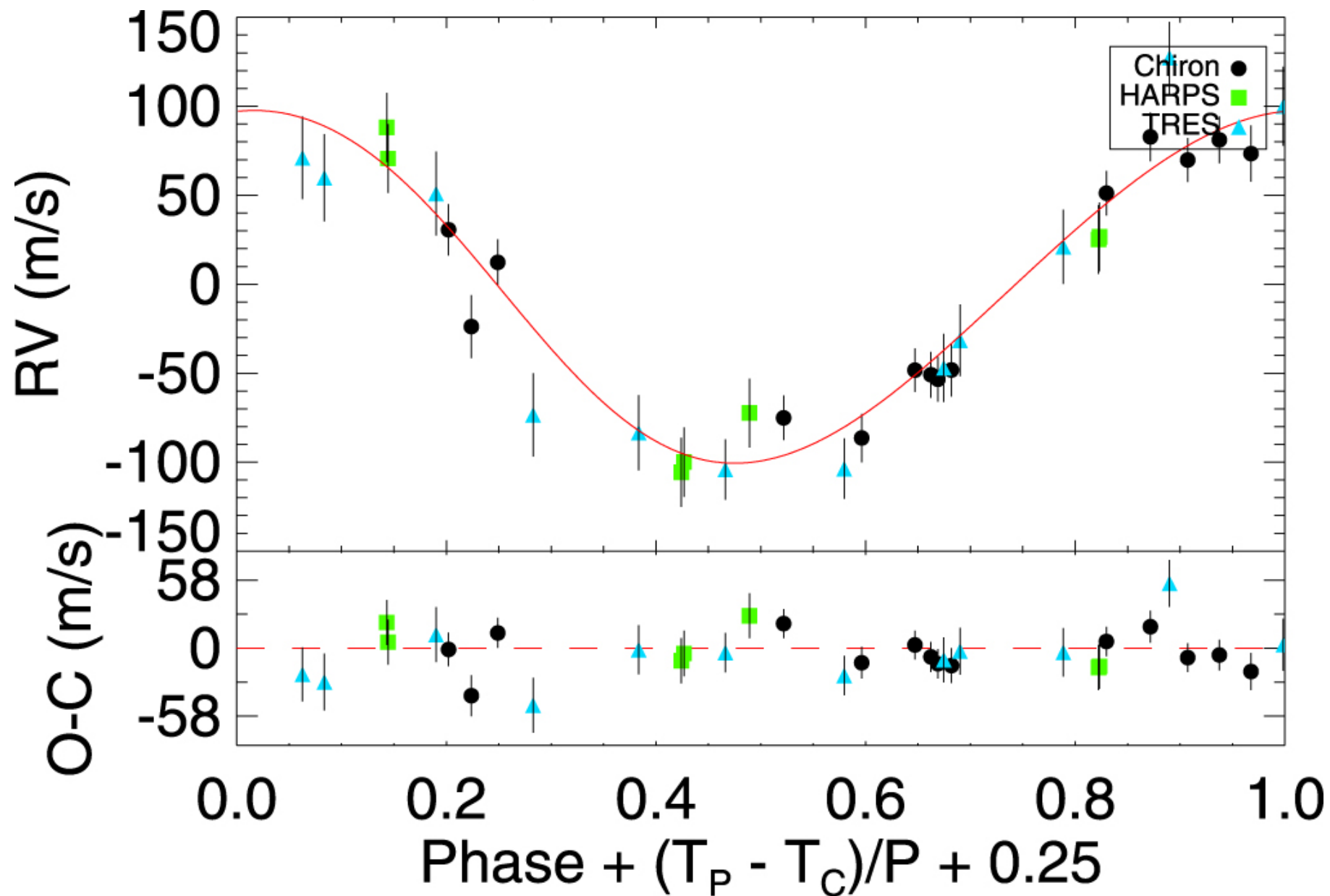
Figure 4. from HD 202772A b: A Transiting Hot Jupiter around a Bright, Mildly Evolved Star in a Visual Binary Discovered by TESS null 2019 AJ 157 51 doi:10.3847/1538-3881/aaf1b7 https://dx.doi.org/10.3847/1538-3881/aaf1b7 © 2019. The American Astronomical Society. All rights reserved.
