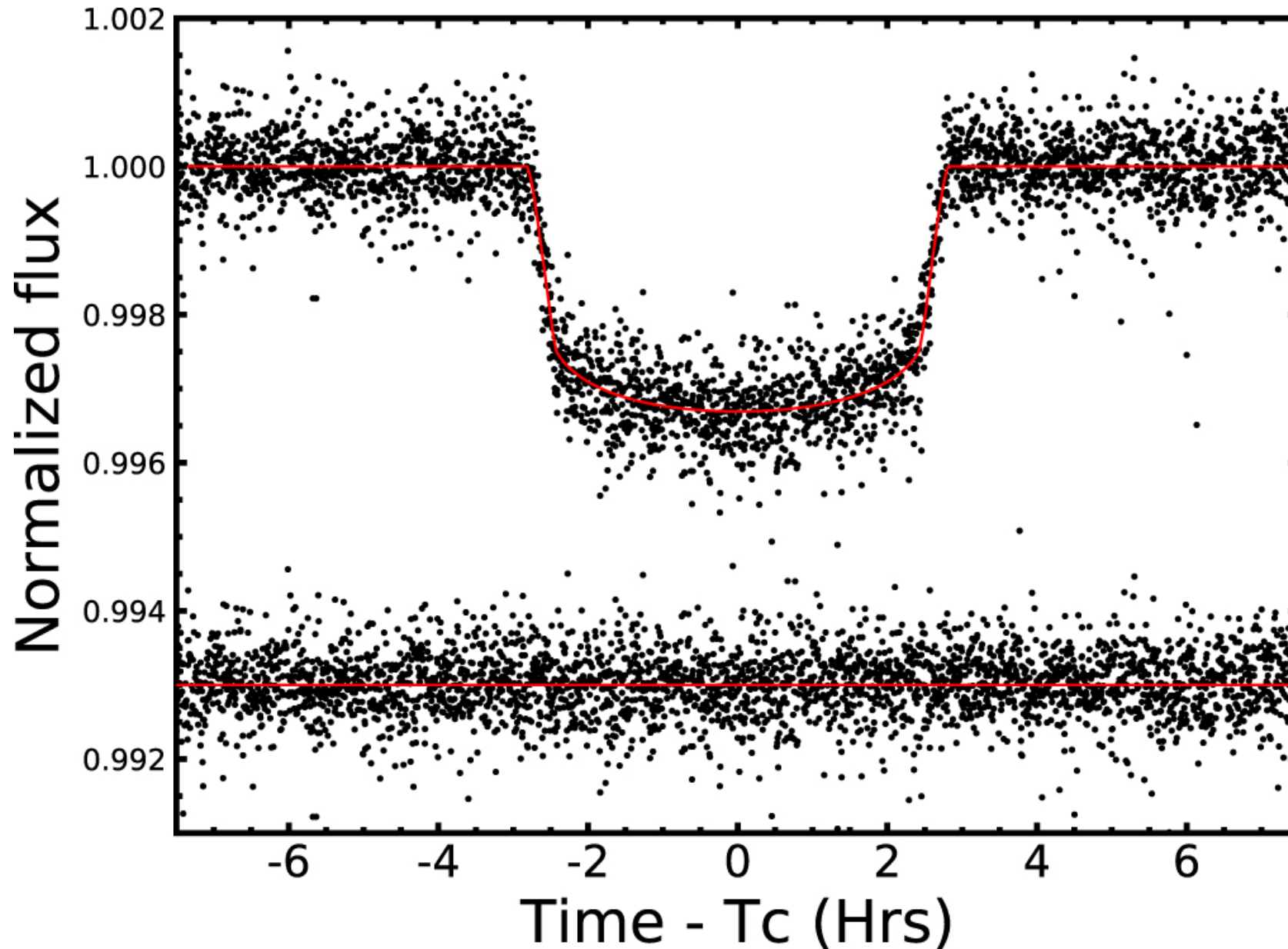
Figure 3. from HD 202772A b: A Transiting Hot Jupiter around a Bright, Mildly Evolved Star in a Visual Binary Discovered by TESS null 2019 AJ 157 51 doi:10.3847/1538-3881/aaf1b7 https://dx.doi.org/10.3847/1538-3881/aaf1b7 © 2019. The American Astronomical Society. All rights reserved.
