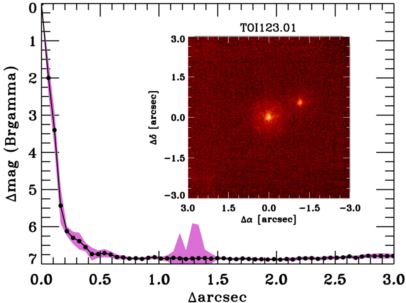
Figure 2. from HD 202772A b: A Transiting Hot Jupiter around a Bright, Mildly Evolved Star in a Visual Binary Discovered by TESS null 2019 AJ 157 51 doi:10.3847/1538-3881/aaf1b7 https://dx.doi.org/10.3847/1538-3881/aaf1b7 © 2019. The American Astronomical Society. All rights reserved.
