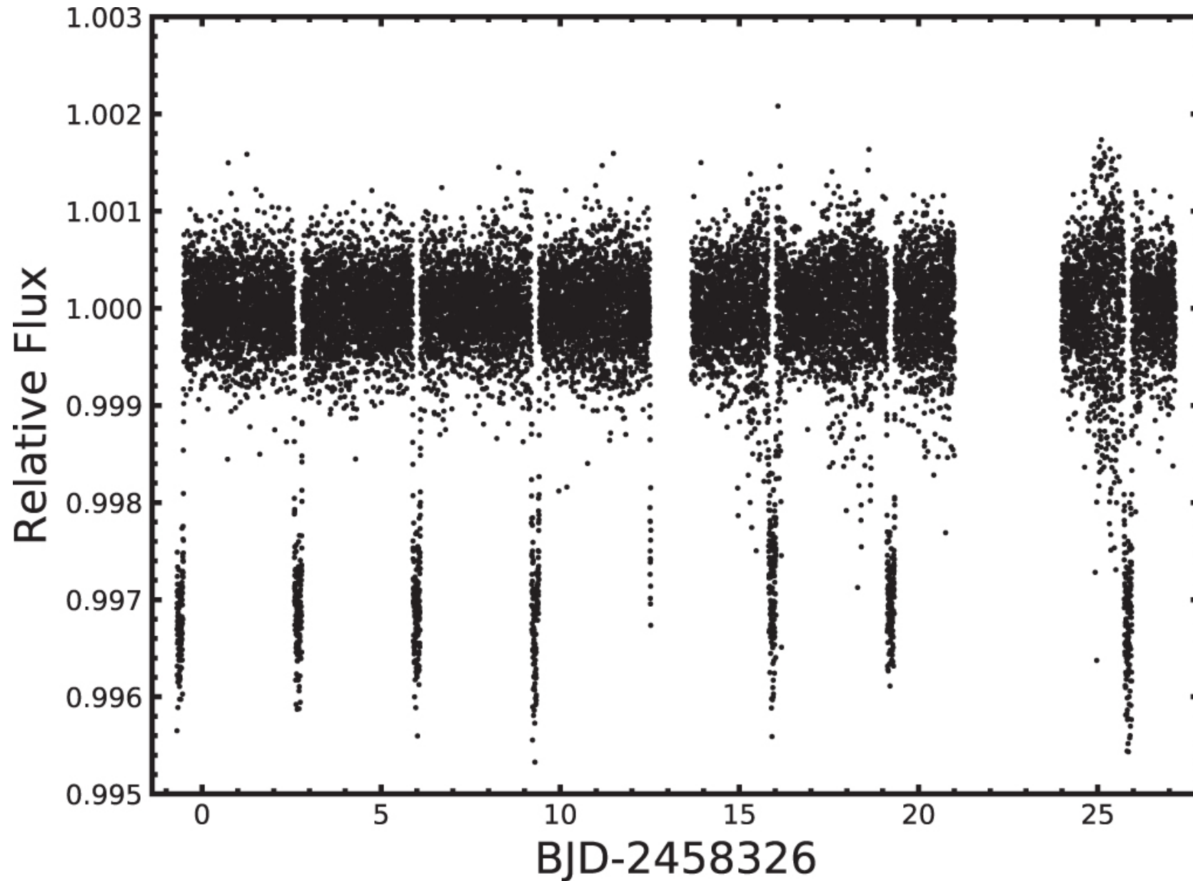
Figure 1. from HD 202772A b: A Transiting Hot Jupiter around a Bright, Mildly Evolved Star in a Visual Binary Discovered by TESS null 2019 AJ 157 51 doi:10.3847/1538-3881/aaf1b7 https://dx.doi.org/10.3847/1538-3881/aaf1b7 © 2019. The American Astronomical Society. All rights reserved.
