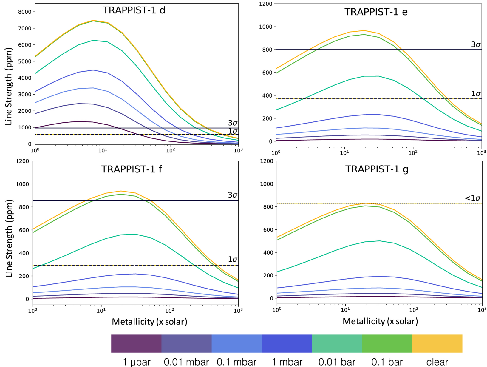
Figure 3. from Limits on Clouds and Hazes for the TRAPPIST-1 Planets null 2018 AJ 156 252 doi:10.3847/1538-3881/aae83a https://dx.doi.org/10.3847/1538-3881/aae83a © 2018. The American Astronomical Society. All rights reserved.
