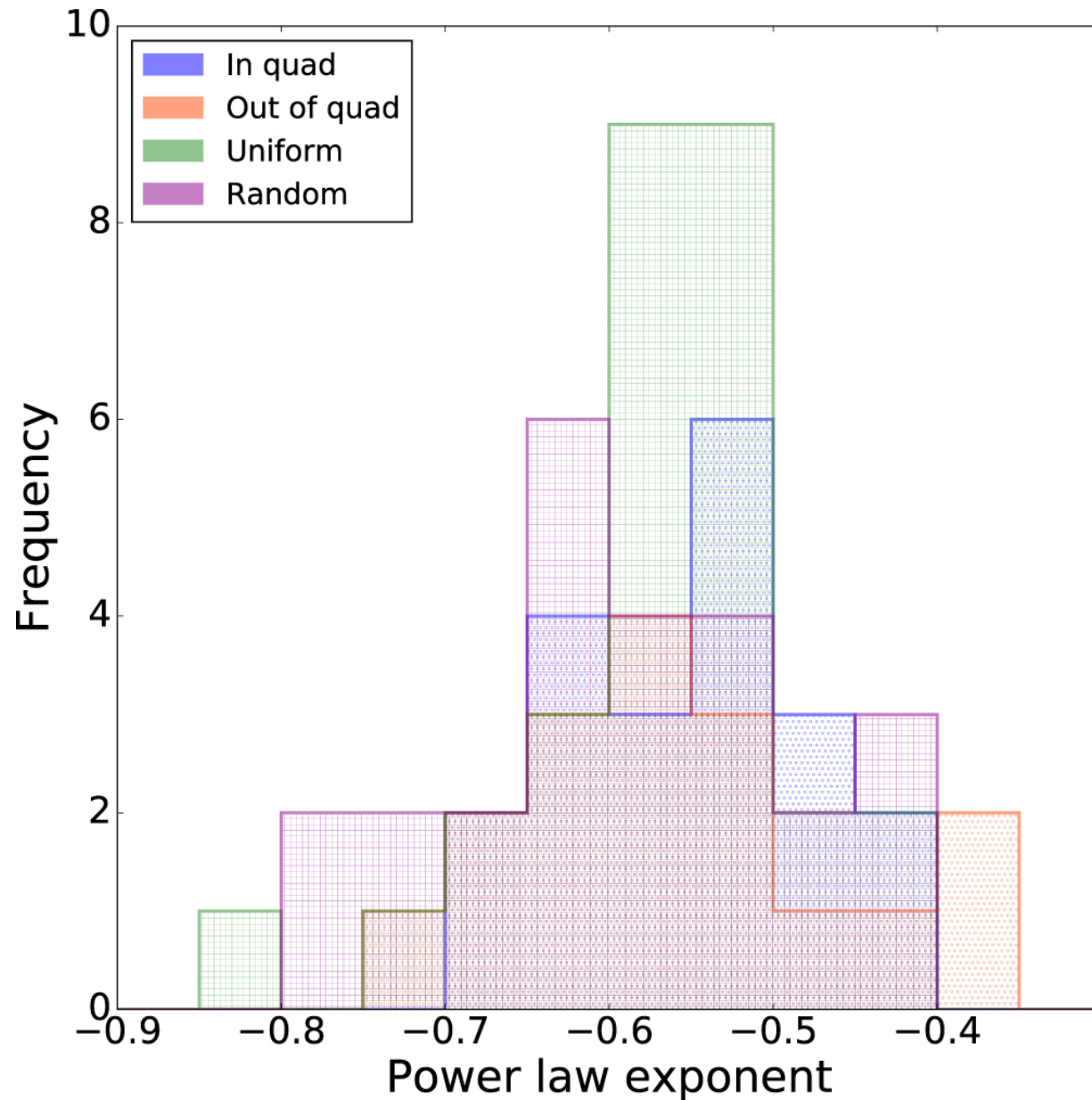
Figure 8. from Simulating the M–R Relation from APF Follow-up of TESS Targets: Survey Design and Strategies for Overcoming Mass Biases null 2018 AJ 156 255 doi:10.3847/1538-3881/aae697 https://dx.doi.org/10.3847/1538-3881/aae697 © 2018. The American Astronomical Society. All rights reserved.
