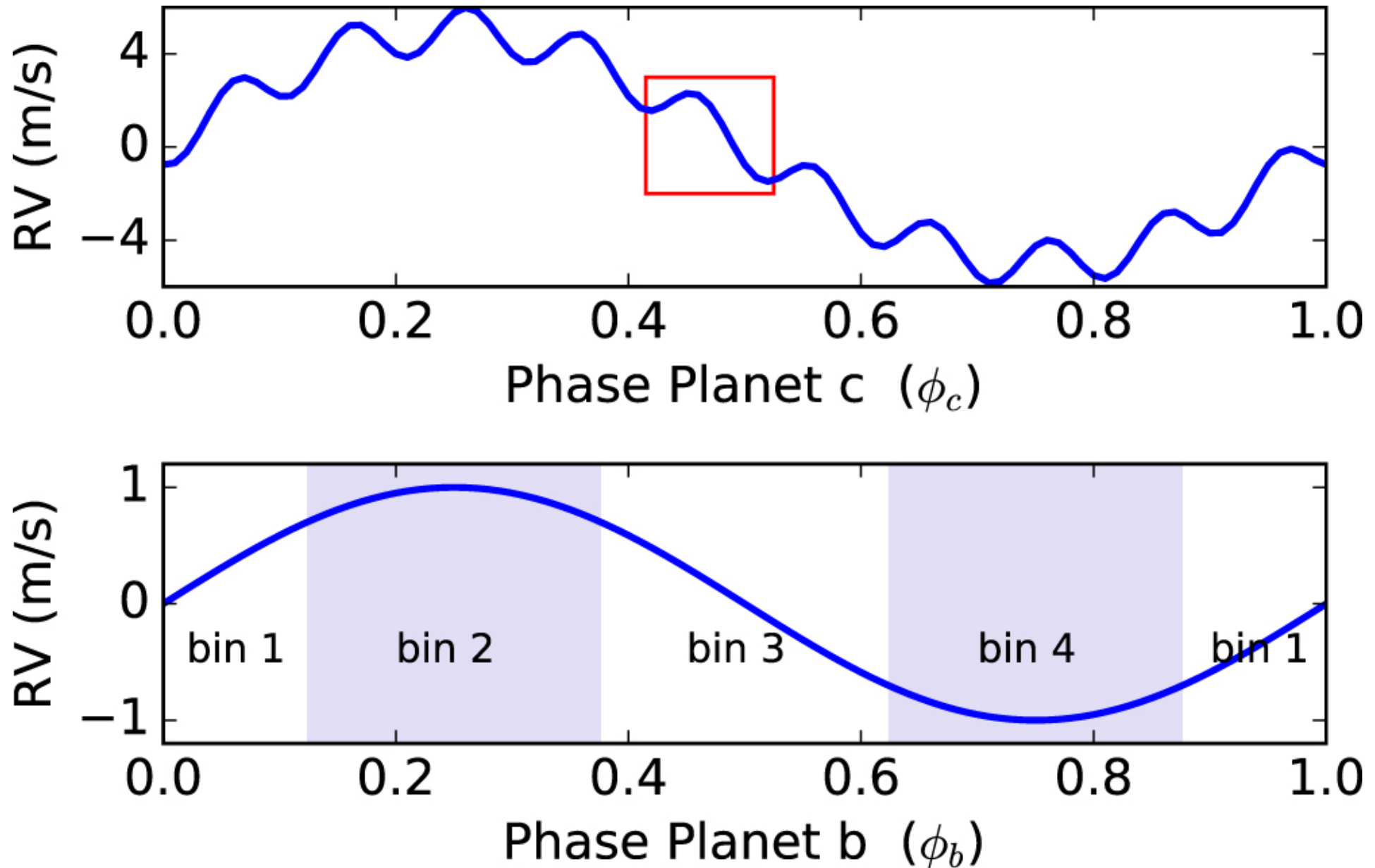
Figure 5. from Simulating the M–R Relation from APF Follow-up of TESS Targets: Survey Design and Strategies for Overcoming Mass Biases null 2018 AJ 156 255 doi:10.3847/1538-3881/aae697 https://dx.doi.org/10.3847/1538-3881/aae697 © 2018. The American Astronomical Society. All rights reserved.
