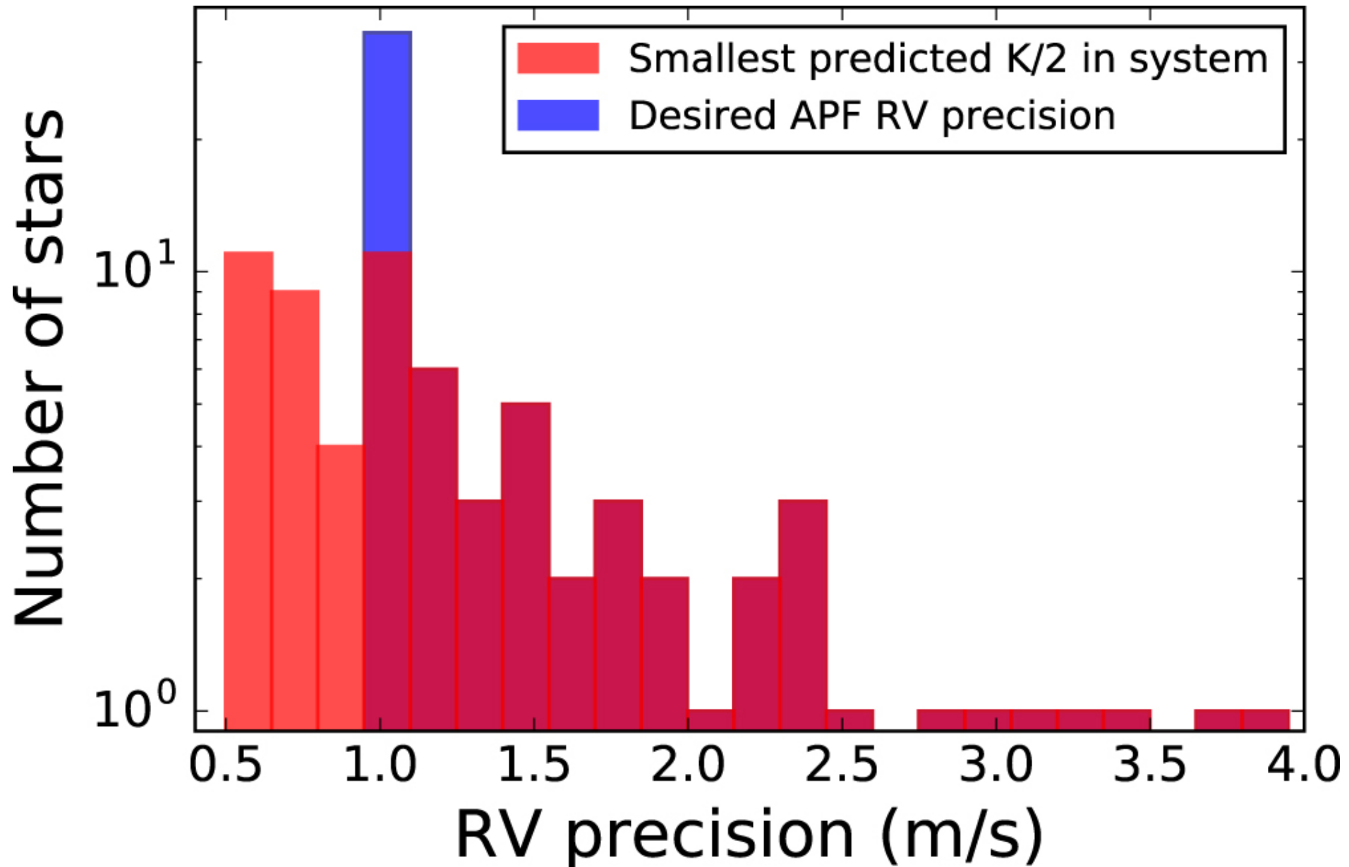
Figure 4. from Simulating the M–R Relation from APF Follow-up of TESS Targets: Survey Design and Strategies for Overcoming Mass Biases null 2018 AJ 156 255 doi:10.3847/1538-3881/aae697 https://dx.doi.org/10.3847/1538-3881/aae697 © 2018. The American Astronomical Society. All rights reserved.
