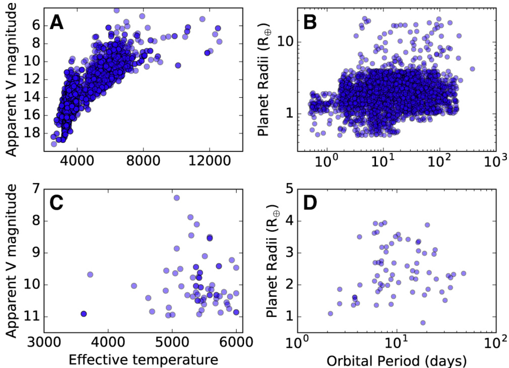
Figure 3. from Simulating the M–R Relation from APF Follow-up of TESS Targets: Survey Design and Strategies for Overcoming Mass Biases null 2018 AJ 156 255 doi:10.3847/1538-3881/aae697 https://dx.doi.org/10.3847/1538-3881/aae697 © 2018. The American Astronomical Society. All rights reserved.
