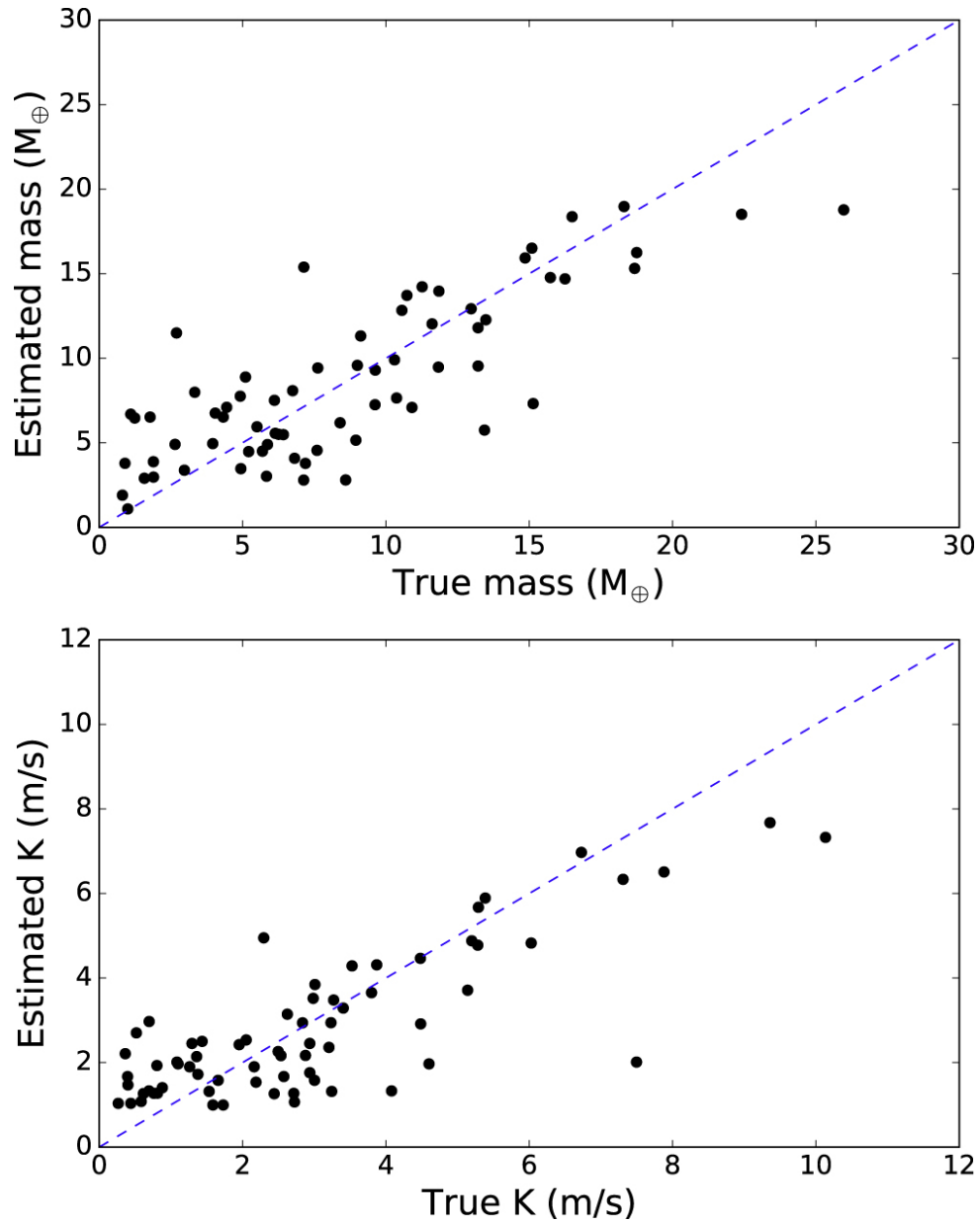
Figure 2. from Simulating the M–R Relation from APF Follow-up of TESS Targets: Survey Design and Strategies for Overcoming Mass Biases null 2018 AJ 156 255 doi:10.3847/1538-3881/aae697 https://dx.doi.org/10.3847/1538-3881/aae697 © 2018. The American Astronomical Society. All rights reserved.
