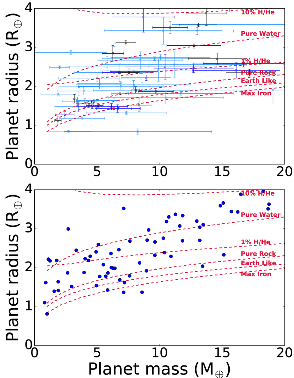
Figure 10. from Simulating the M–R Relation from APF Follow-up of TESS Targets: Survey Design and Strategies for Overcoming Mass Biases null 2018 AJ 156 255 doi:10.3847/1538-3881/aae697 https://dx.doi.org/10.3847/1538-3881/aae697 © 2018. The American Astronomical Society. All rights reserved.
