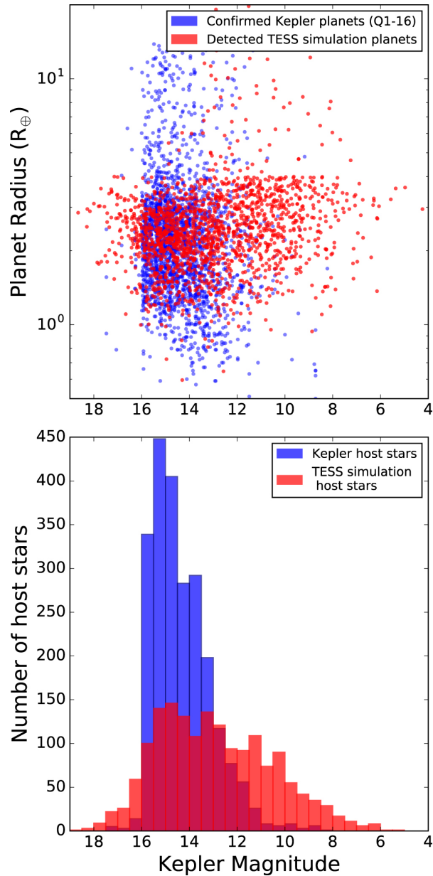
Figure 1. from Simulating the M–R Relation from APF Follow-up of TESS Targets: Survey Design and Strategies for Overcoming Mass Biases null 2018 AJ 156 255 doi:10.3847/1538-3881/aae697 https://dx.doi.org/10.3847/1538-3881/aae697 © 2018. The American Astronomical Society. All rights reserved.
