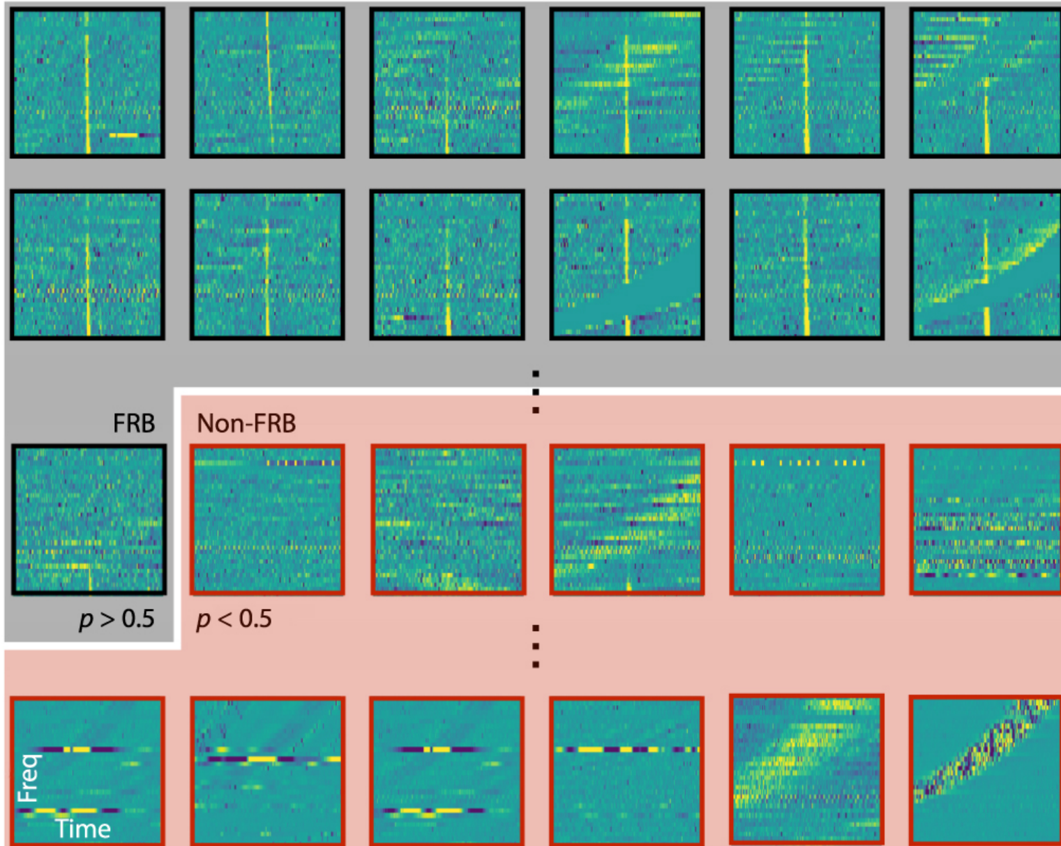
Figure 8. from Applying Deep Learning to Fast Radio Burst Classification null 2018 AJ 156 256 doi:10.3847/1538-3881/aae649 https://dx.doi.org/10.3847/1538-3881/aae649 © 2018. The American Astronomical Society. All rights reserved.
