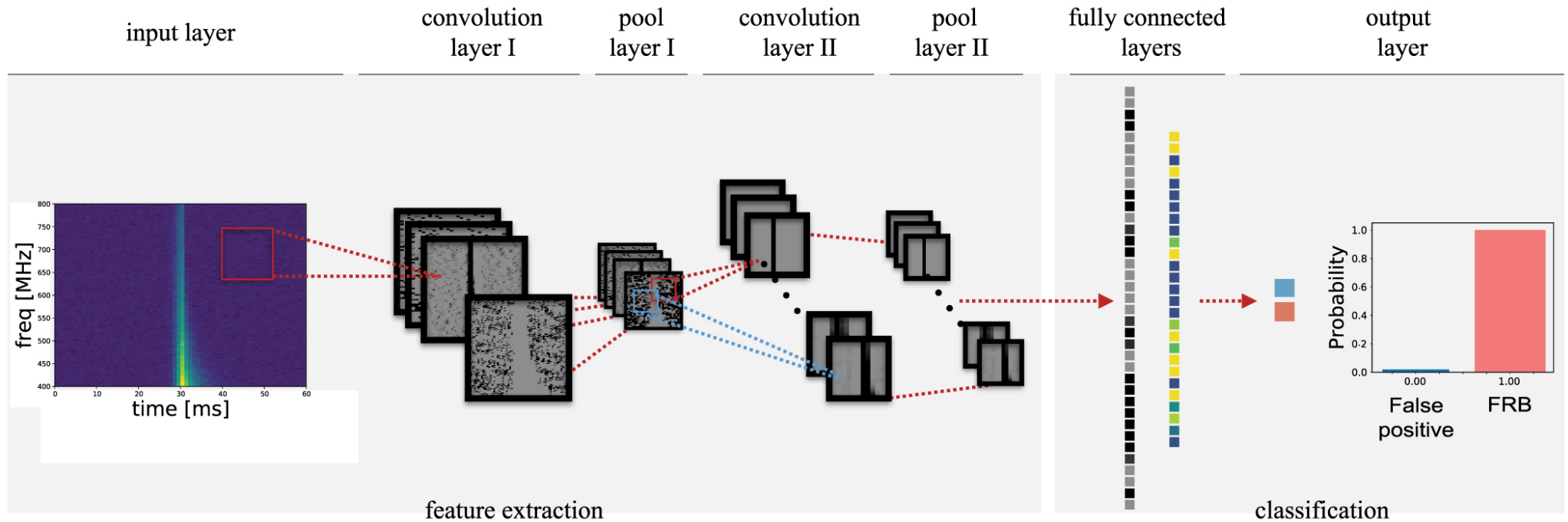
Figure 3. from Applying Deep Learning to Fast Radio Burst Classification null 2018 AJ 156 256 doi:10.3847/1538-3881/aae649 https://dx.doi.org/10.3847/1538-3881/aae649 © 2018. The American Astronomical Society. All rights reserved.
