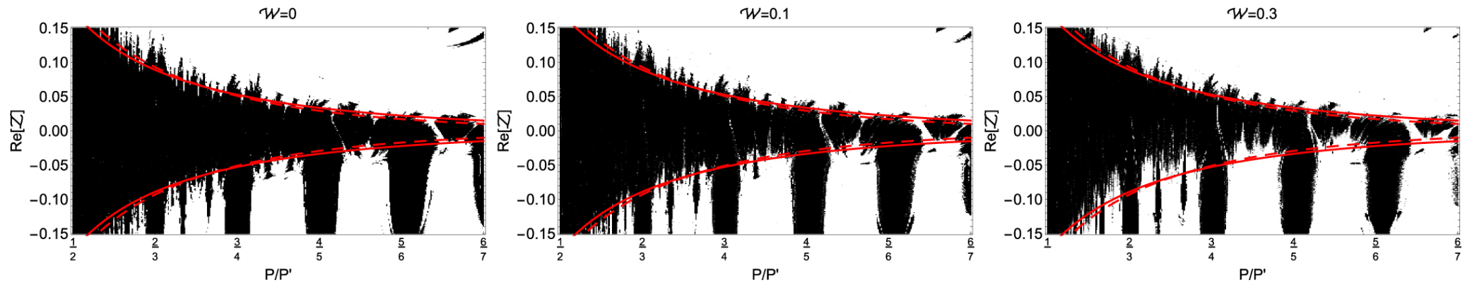
Figure 6. from A Criterion for the Onset of Chaos in Systems of Two Eccentric Planets null 2018 AJ 156 95 doi:10.3847/1538-3881/aad32c https://dx.doi.org/10.3847/1538-3881/aad32c © 2018. The American Astronomical Society. All rights reserved.
