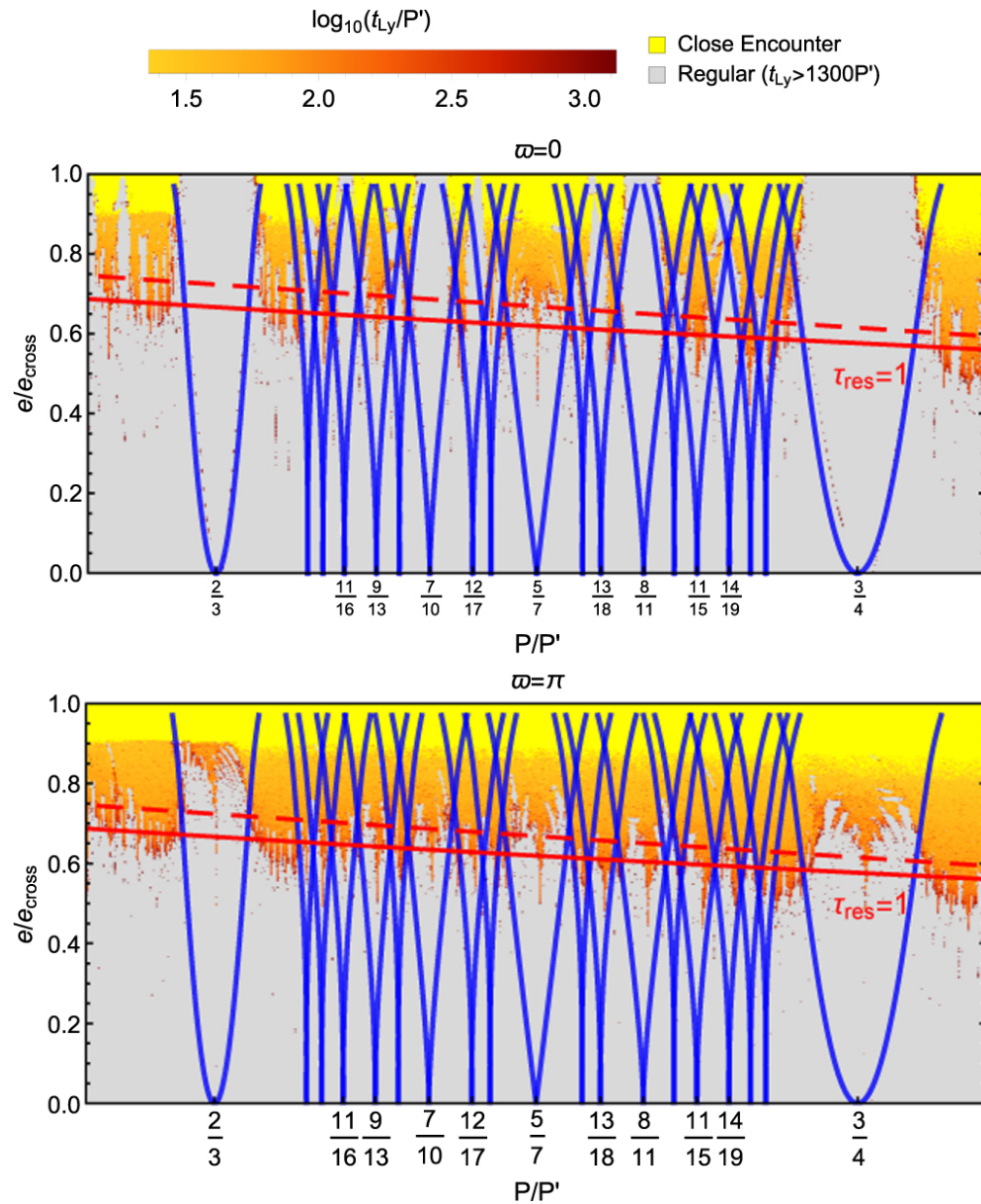
Figure 5. from A Criterion for the Onset of Chaos in Systems of Two Eccentric Planets null 2018 AJ 156 95 doi:10.3847/1538-3881/aad32c https://dx.doi.org/10.3847/1538-3881/aad32c © 2018. The American Astronomical Society. All rights reserved.
