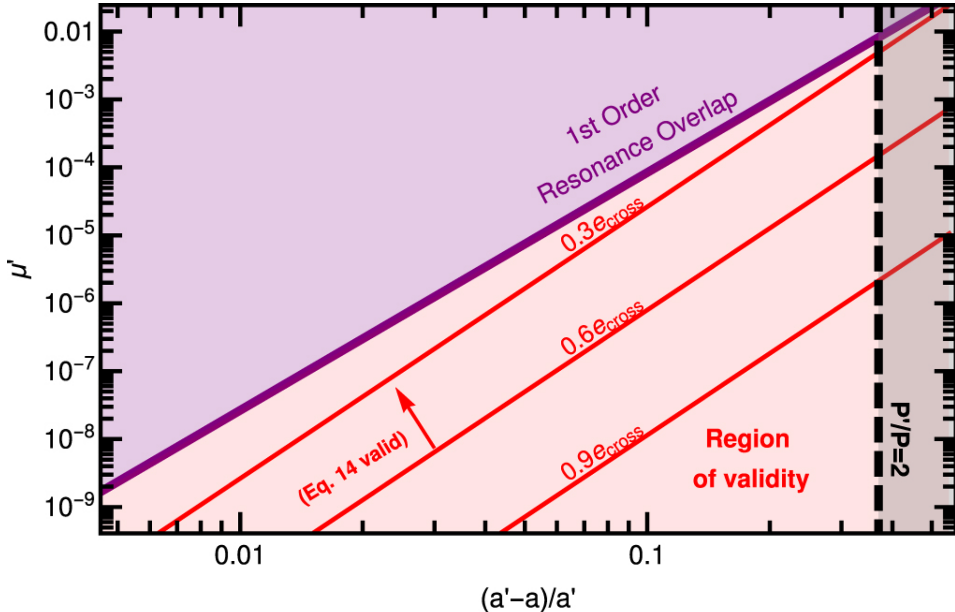
Figure 4. from A Criterion for the Onset of Chaos in Systems of Two Eccentric Planets null 2018 AJ 156 95 doi:10.3847/1538-3881/aad32c https://dx.doi.org/10.3847/1538-3881/aad32c © 2018. The American Astronomical Society. All rights reserved.
