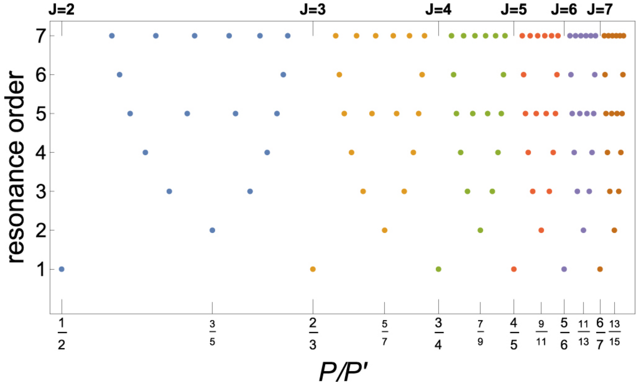
Figure 2. from A Criterion for the Onset of Chaos in Systems of Two Eccentric Planets null 2018 AJ 156 95 doi:10.3847/1538-3881/aad32c https://dx.doi.org/10.3847/1538-3881/aad32c © 2018. The American Astronomical Society. All rights reserved.
