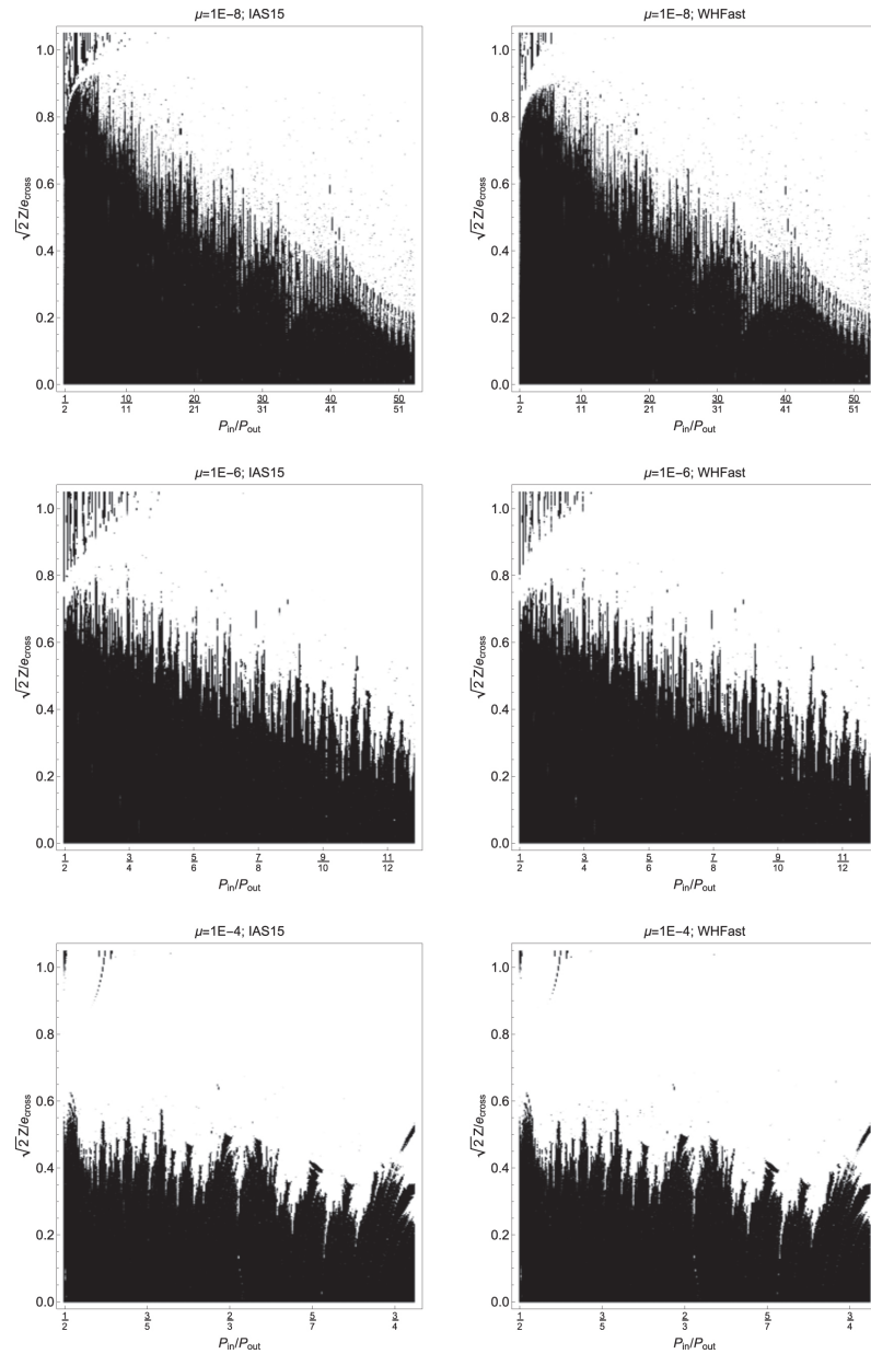
Figure 13. from A Criterion for the Onset of Chaos in Systems of Two Eccentric Planets null 2018 AJ 156 95 doi:10.3847/1538-3881/aad32c https://dx.doi.org/10.3847/1538-3881/aad32c © 2018. The American Astronomical Society. All rights reserved.
