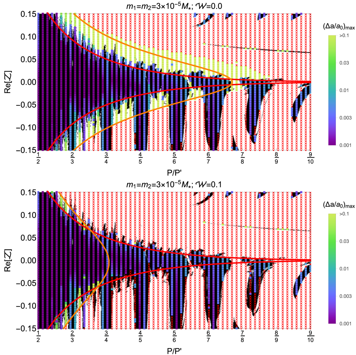
Figure 11. from A Criterion for the Onset of Chaos in Systems of Two Eccentric Planets null 2018 AJ 156 95 doi:10.3847/1538-3881/aad32c https://dx.doi.org/10.3847/1538-3881/aad32c © 2018. The American Astronomical Society. All rights reserved.
