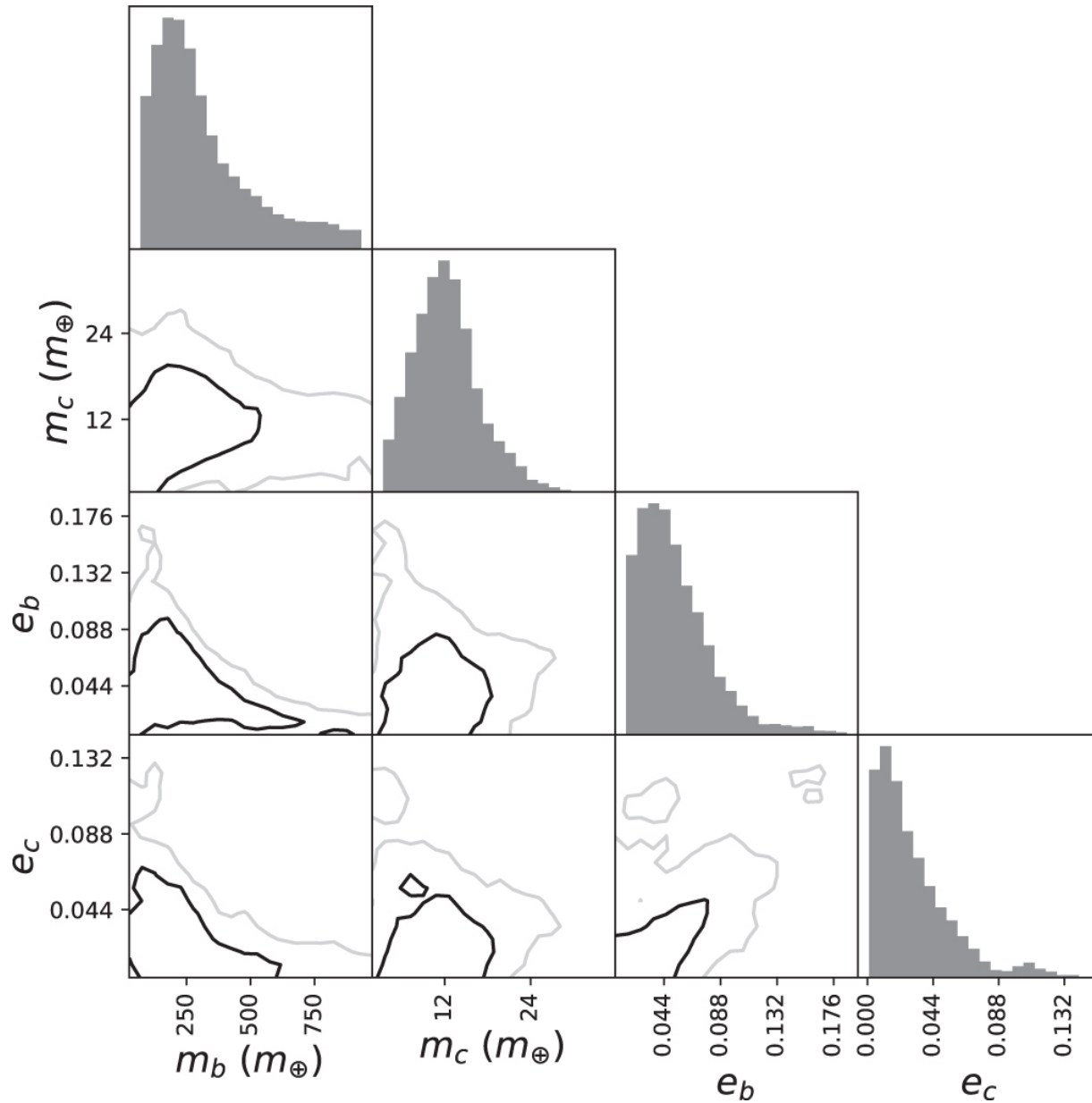
Figure 10. from TTV-determined Masses for Warm Jupiters and Their Close Planetary Companions null 2018 AJ 156 96 doi:10.3847/1538-3881/aad22b https://dx.doi.org/10.3847/1538-3881/aad22b © 2018. The American Astronomical Society. All rights reserved.
