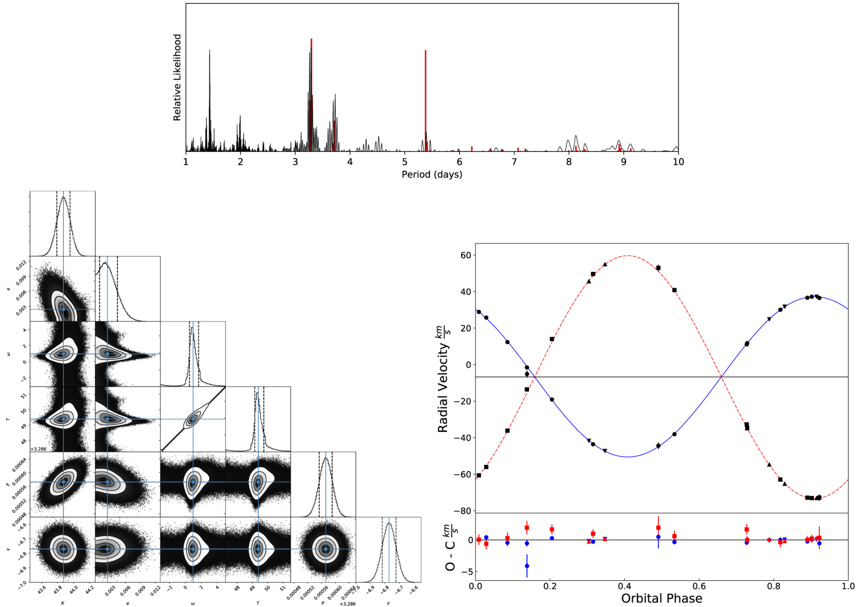
Figure 9. from Forty-four New and Known M-dwarf Multiples in the SDSS-III/APOGEE M-dwarf Ancillary Science Sample null 2018 AJ 156 45 doi:10.3847/1538-3881/aac9c2 https://dx.doi.org/10.3847/1538-3881/aac9c2 © 2018. The American Astronomical Society. All rights reserved.
