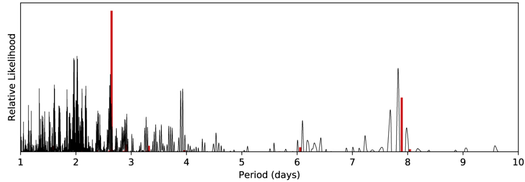
Figure 8. from Forty-four New and Known M-dwarf Multiples in the SDSS-III/APOGEE M-dwarf Ancillary Science Sample null 2018 AJ 156 45 doi:10.3847/1538-3881/aac9c2 https://dx.doi.org/10.3847/1538-3881/aac9c2 © 2018. The American Astronomical Society. All rights reserved.
