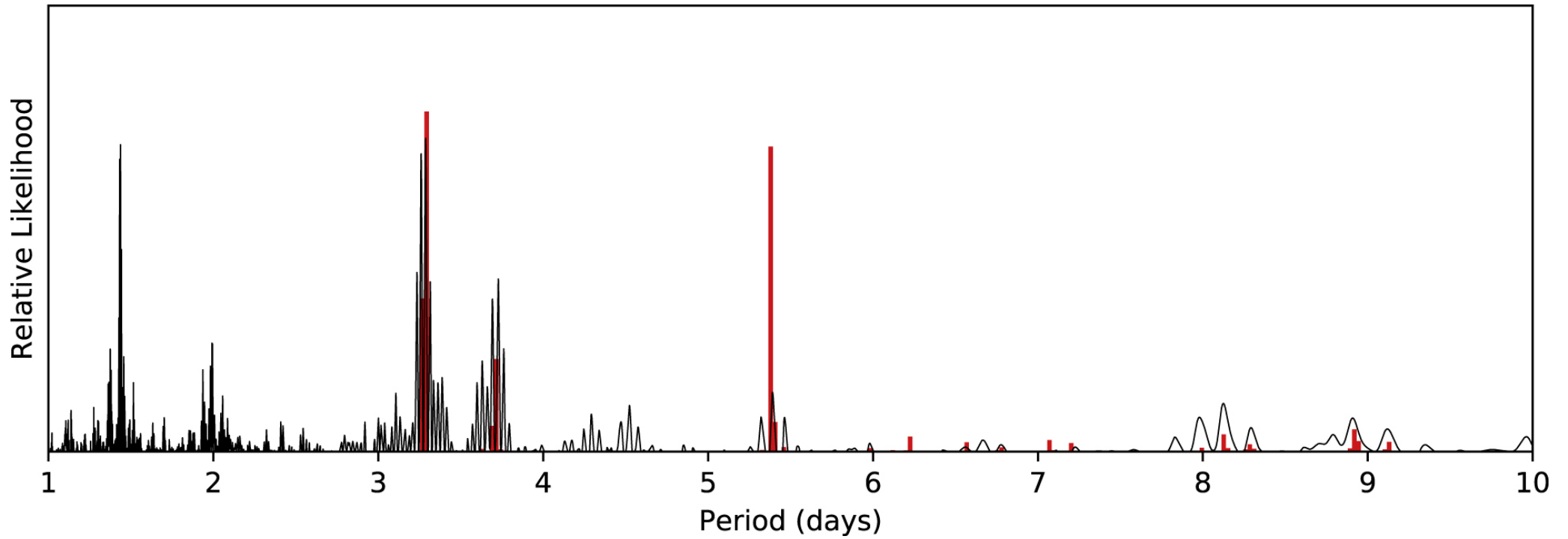
Figure 7. from Forty-four New and Known M-dwarf Multiples in the SDSS-III/APOGEE M-dwarf Ancillary Science Sample null 2018 AJ 156 45 doi:10.3847/1538-3881/aac9c2 https://dx.doi.org/10.3847/1538-3881/aac9c2 © 2018. The American Astronomical Society. All rights reserved.
