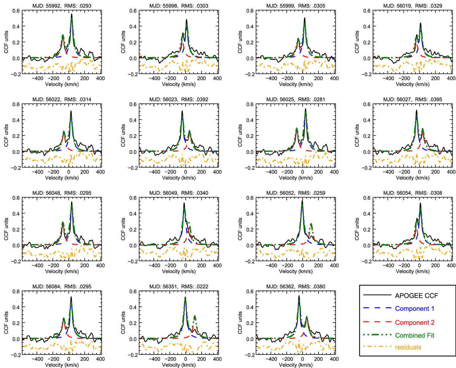
Figure 3. from Forty-four New and Known M-dwarf Multiples in the SDSS-III/APOGEE M-dwarf Ancillary Science Sample null 2018 AJ 156 45 doi:10.3847/1538-3881/aac9c2 https://dx.doi.org/10.3847/1538-3881/aac9c2
