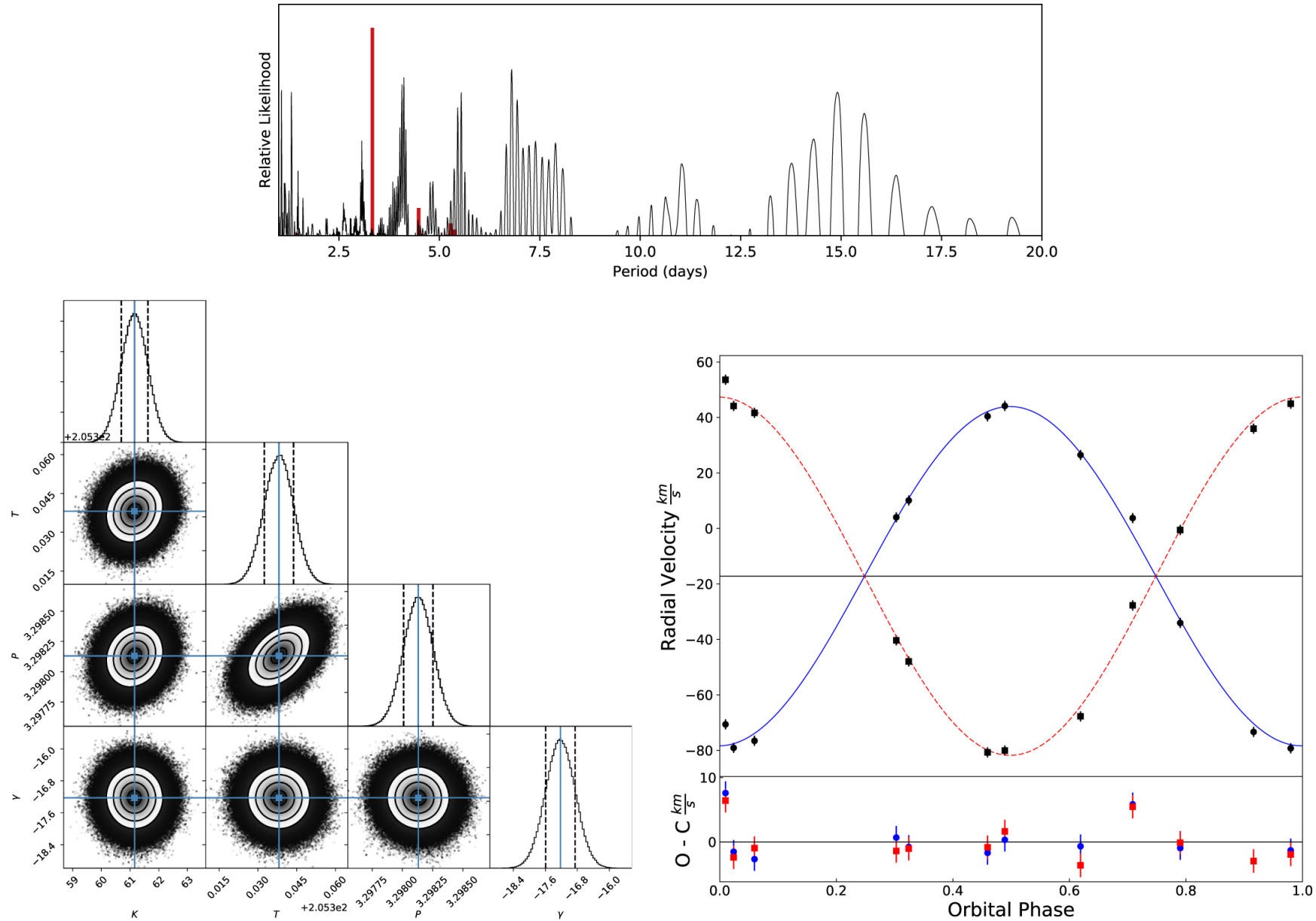
Figure 11. from Forty-four New and Known M-dwarf Multiples in the SDSS-III/APOGEE M-dwarf Ancillary Science Sample null 2018 AJ 156 45 doi:10.3847/1538-3881/aac9c2 https://dx.doi.org/10.3847/1538-3881/aac9c2 © 2018. The American Astronomical Society. All rights reserved.
