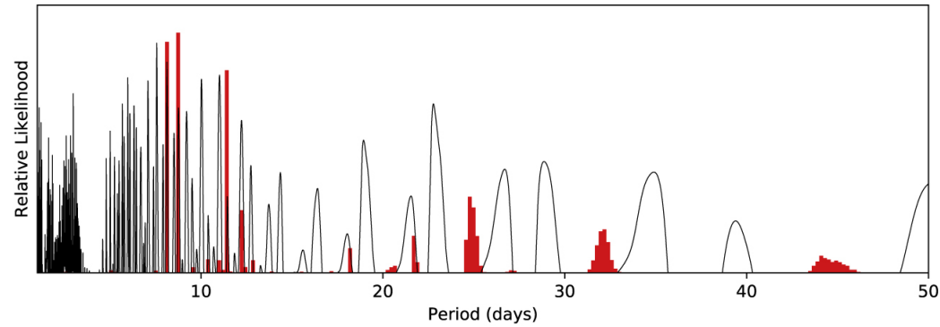
Figure 10. from Forty-four New and Known M-dwarf Multiples in the SDSS-III/APOGEE M-dwarf Ancillary Science Sample null 2018 AJ 156 45 doi:10.3847/1538-3881/aac9c2 https://dx.doi.org/10.3847/1538-3881/aac9c2 © 2018. The American Astronomical Society. All rights reserved.
