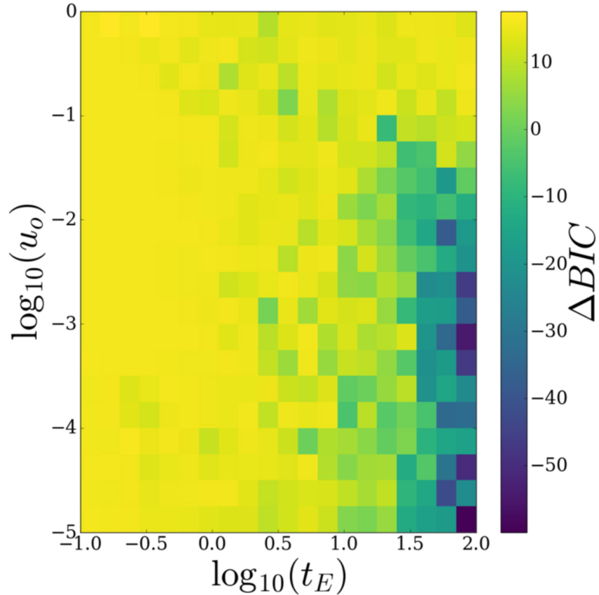
Figure 5. from Measuring the Microlensing Parallax from Various Space Observatories null 2018 AJ 155 191 doi:10.3847/1538-3881/aab3c8 https://dx.doi.org/10.3847/1538-3881/aab3c8 © 2018. The American Astronomical Society. All rights reserved.
