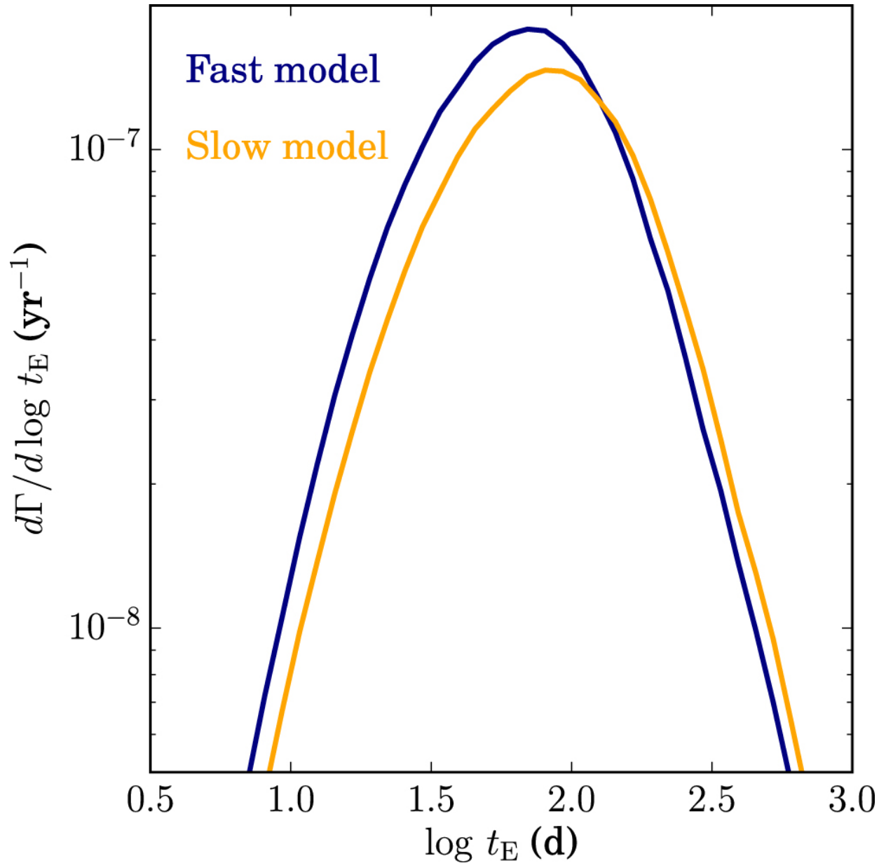
Figure 3. from New Self-lensing Models of the Small Magellanic Cloud: Can Gravitational Microlensing Detect Extragalactic Exoplanets? null 2018 AJ 155 154 doi:10.3847/1538-3881/aab203 https://dx.doi.org/10.3847/1538-3881/aab203 © 2018. The American Astronomical Society. All rights reserved.
