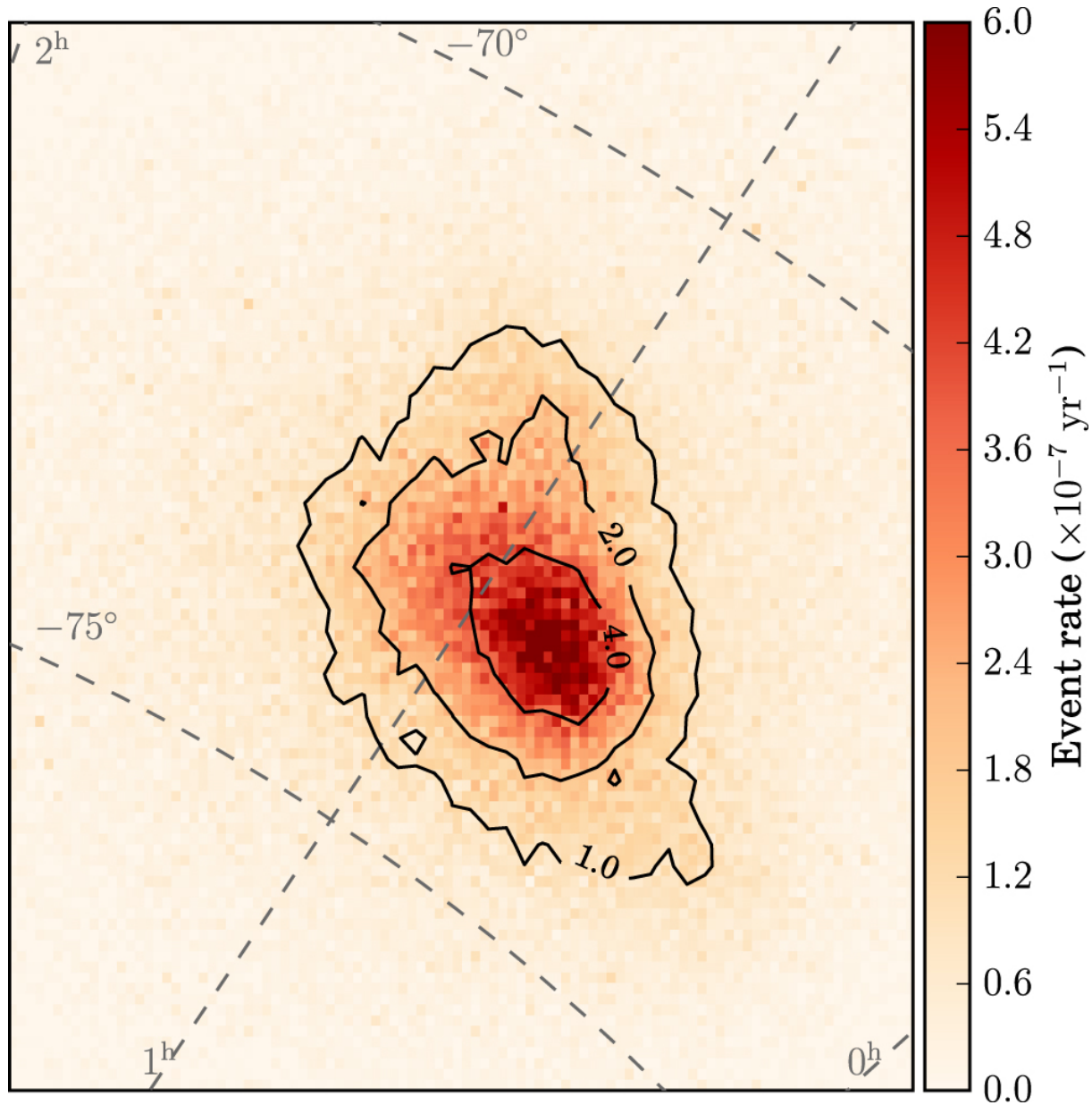
Figure 2. from New Self-lensing Models of the Small Magellanic Cloud: Can Gravitational Microlensing Detect Extragalactic Exoplanets? null 2018 AJ 155 154 doi:10.3847/1538-3881/aab203 https://dx.doi.org/10.3847/1538-3881/aab203 © 2018. The American Astronomical Society. All rights reserved.
