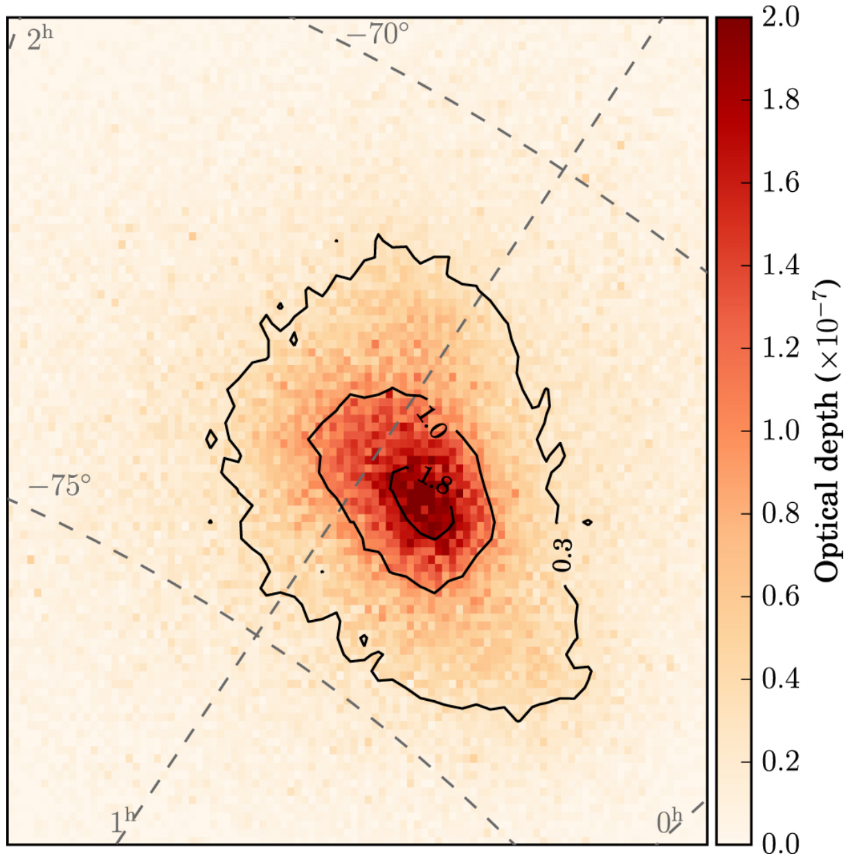
Figure 1. from New Self-lensing Models of the Small Magellanic Cloud: Can Gravitational Microlensing Detect Extragalactic Exoplanets? null 2018 AJ 155 154 doi:10.3847/1538-3881/aab203 https://dx.doi.org/10.3847/1538-3881/aab203 © 2018. The American Astronomical Society. All rights reserved.
