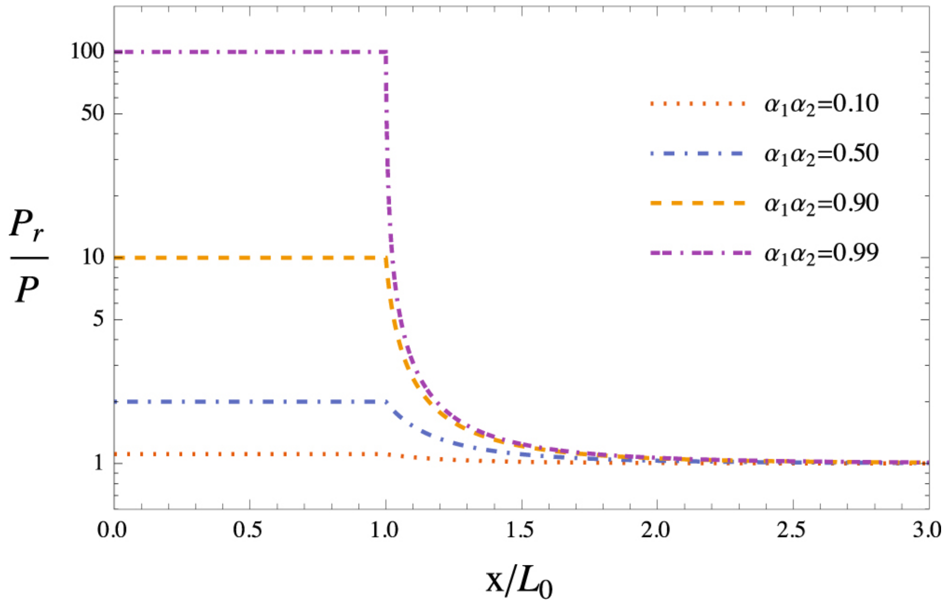
Figure 7. from Relativistic Spacecraft Propelled by Directed Energy null 2018 AJ 155 155 doi:10.3847/1538-3881/aaafd2 https://dx.doi.org/10.3847/1538-3881/aaafd2 © 2018. The American Astronomical Society. All rights reserved.
