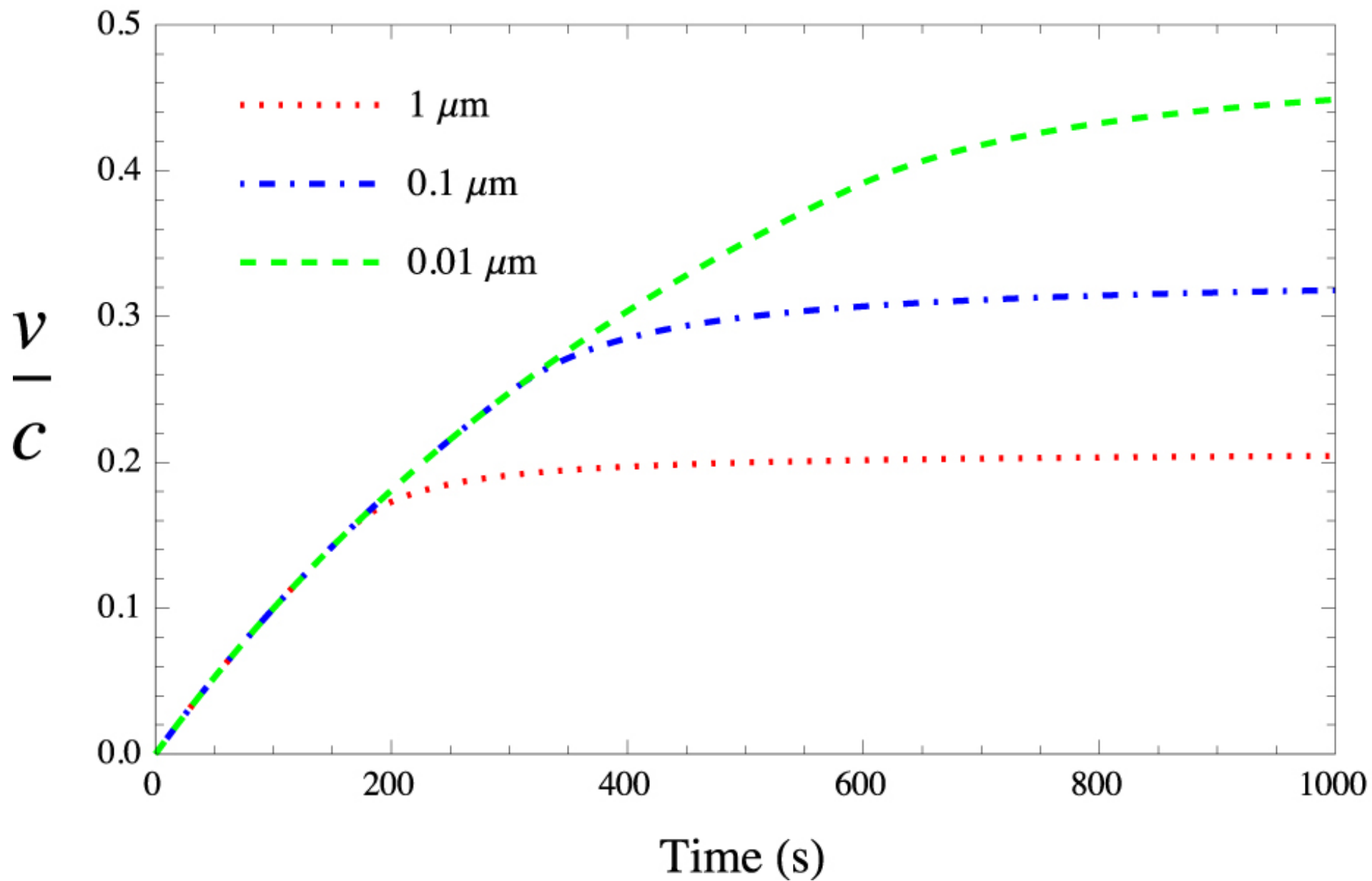
Figure 6. from Relativistic Spacecraft Propelled by Directed Energy null 2018 AJ 155 155 doi:10.3847/1538-3881/aaafd2 https://dx.doi.org/10.3847/1538-3881/aaafd2 © 2018. The American Astronomical Society. All rights reserved.
