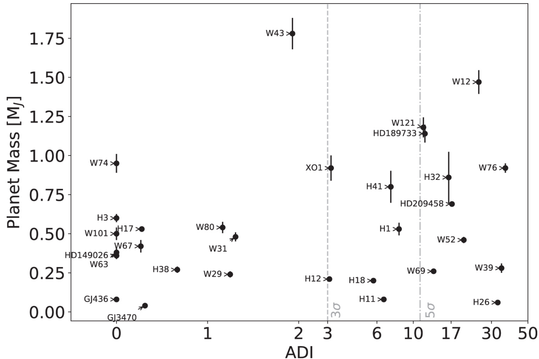
Figure 8. from A Population Study of Gaseous Exoplanets null 2018 AJ 155 156 doi:10.3847/1538-3881/aaaf75 https://dx.doi.org/10.3847/1538-3881/aaaf75 © 2018. The American Astronomical Society.
