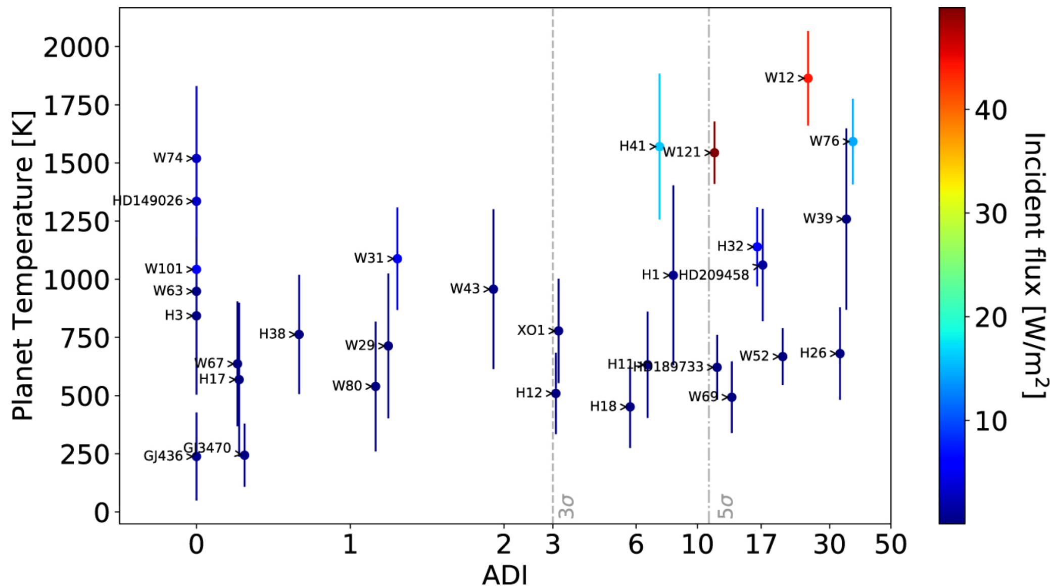
Figure 7. from A Population Study of Gaseous Exoplanets null 2018 AJ 155 156 doi:10.3847/1538-3881/aaaf75 https://dx.doi.org/10.3847/1538-3881/aaaf75 © 2018. The American Astronomical Society.
