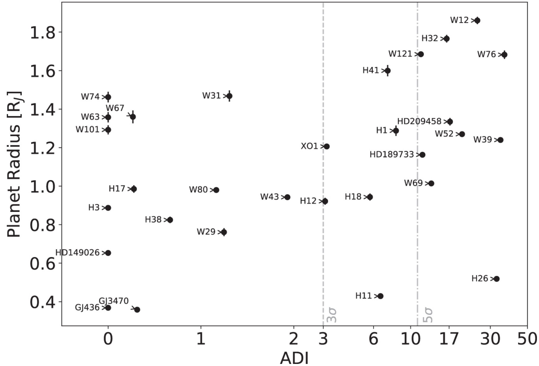
Figure 6. from A Population Study of Gaseous Exoplanets null 2018 AJ 155 156 doi:10.3847/1538-3881/aaaf75 https://dx.doi.org/10.3847/1538-3881/aaaf75 © 2018. The American Astronomical Society.
