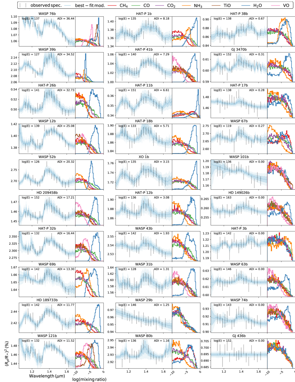
Figure 4. from A Population Study of Gaseous Exoplanets null 2018 AJ 155 156 doi:10.3847/1538-3881/aaaf75 https://dx.doi.org/10.3847/1538-3881/aaaf75 © 2018. The American Astronomical Society.
