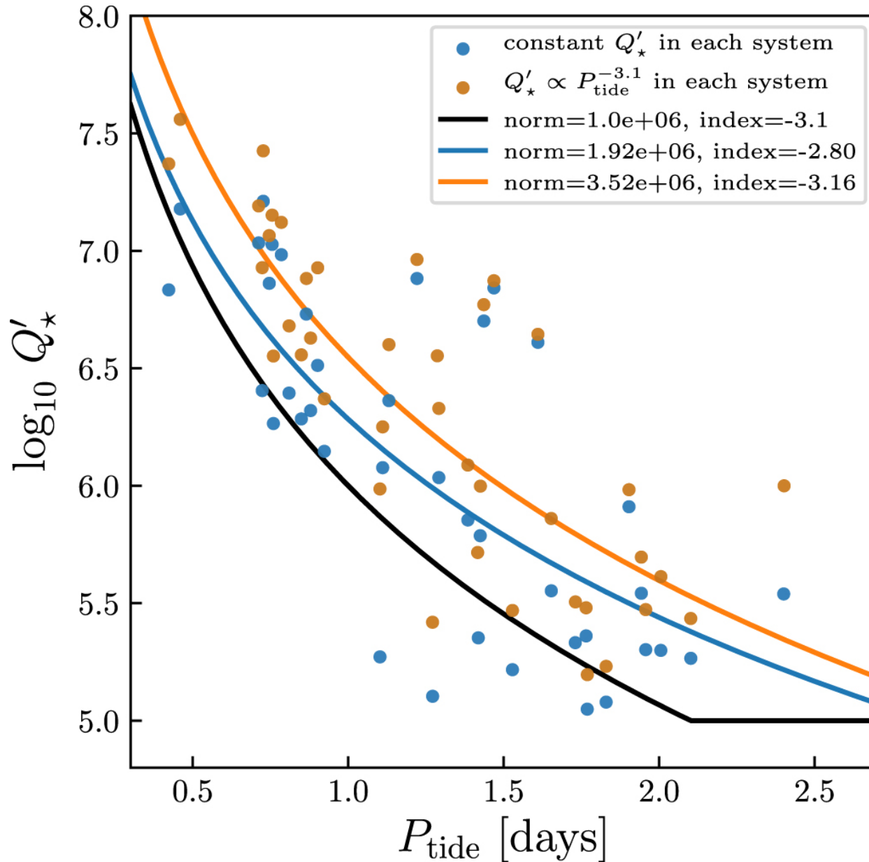
Figure 5. from Empirical Tidal Dissipation in Exoplanet Hosts From Tidal Spin-up null 2018 AJ 155 165 doi:10.3847/1538-3881/aaaf71 https://dx.doi.org/10.3847/1538-3881/aaaf71 © 2018. The American Astronomical Society. All rights reserved.
