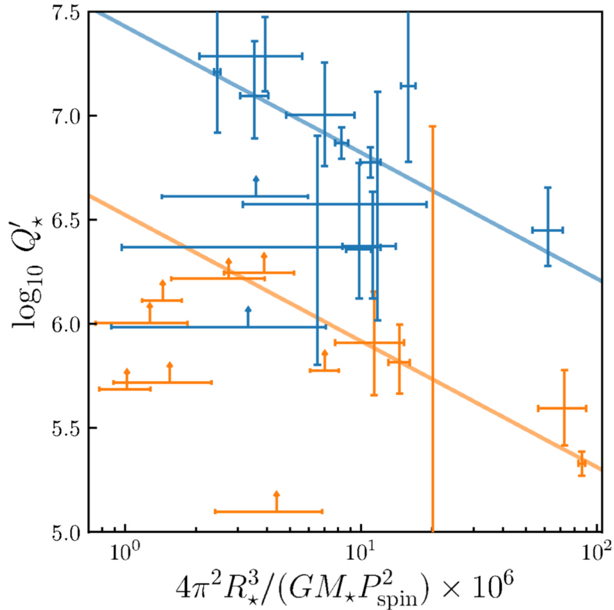
Figure 3. from Empirical Tidal Dissipation in Exoplanet Hosts From Tidal Spin-up null 2018 AJ 155 165 doi:10.3847/1538-3881/aaaf71 https://dx.doi.org/10.3847/1538-3881/aaaf71 © 2018. The American Astronomical Society. All rights reserved.
