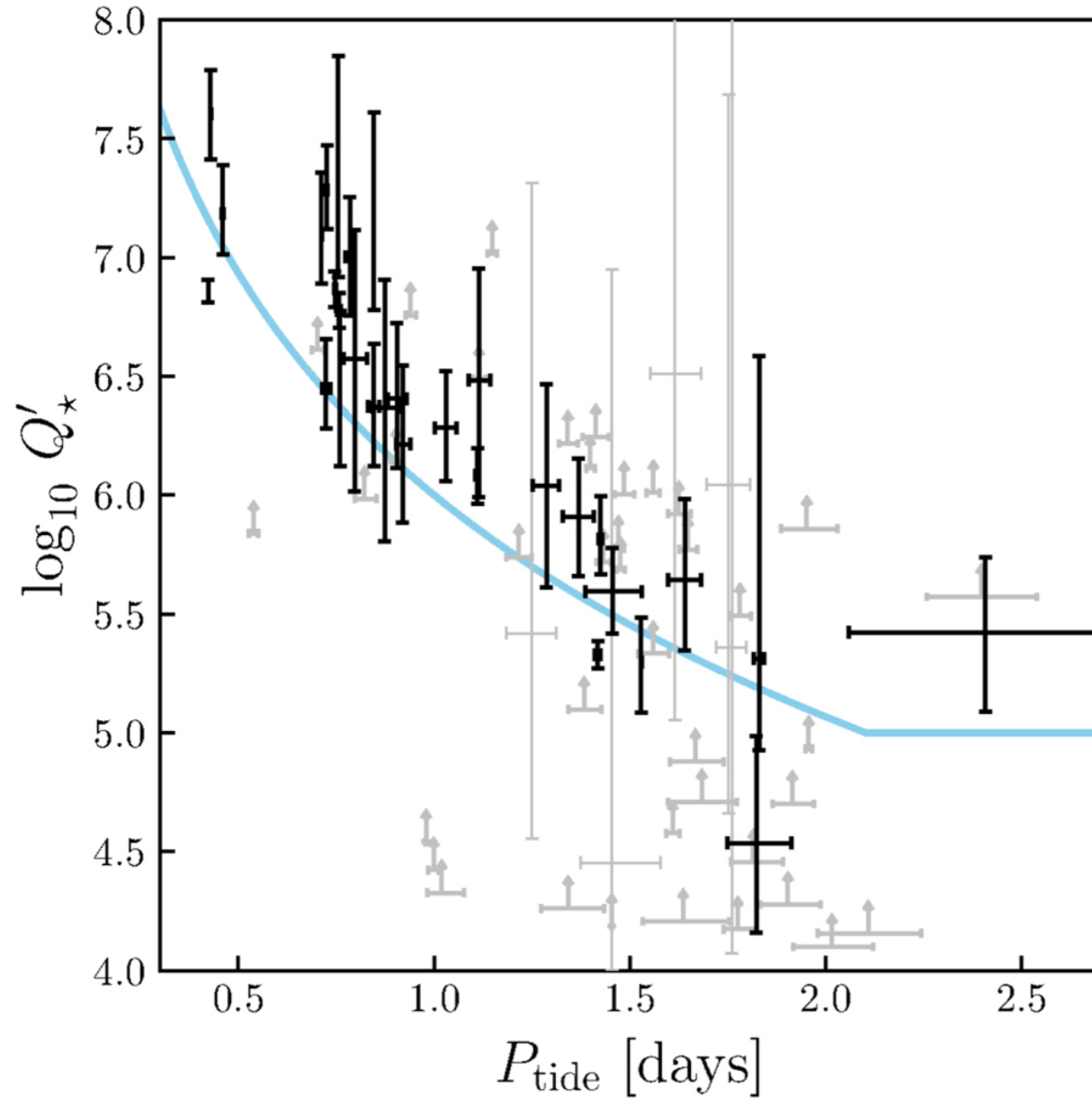
Figure 2. from Empirical Tidal Dissipation in Exoplanet Hosts From Tidal Spin-up null 2018 AJ 155 165 doi:10.3847/1538-3881/aaaf71 https://dx.doi.org/10.3847/1538-3881/aaaf71 © 2018. The American Astronomical Society. All rights reserved.
